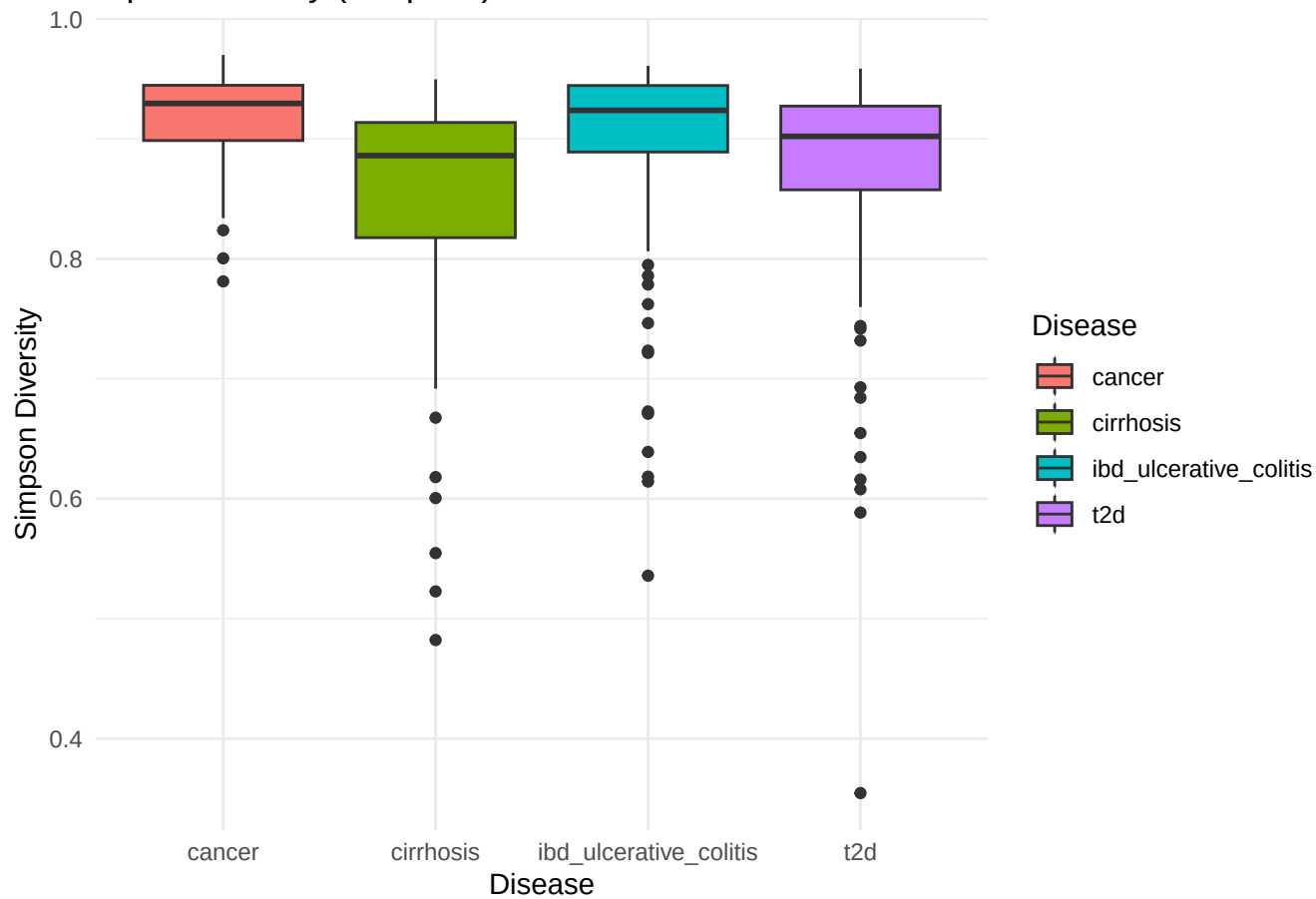
Alpha Diversity (Simpson)
