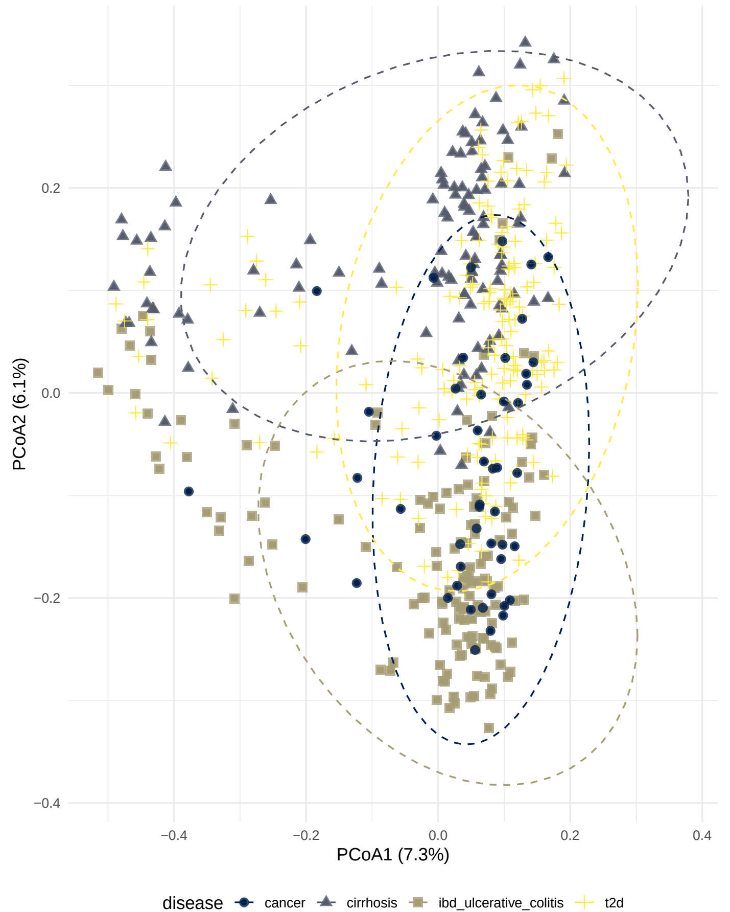
Jaccard Dissimilarity
