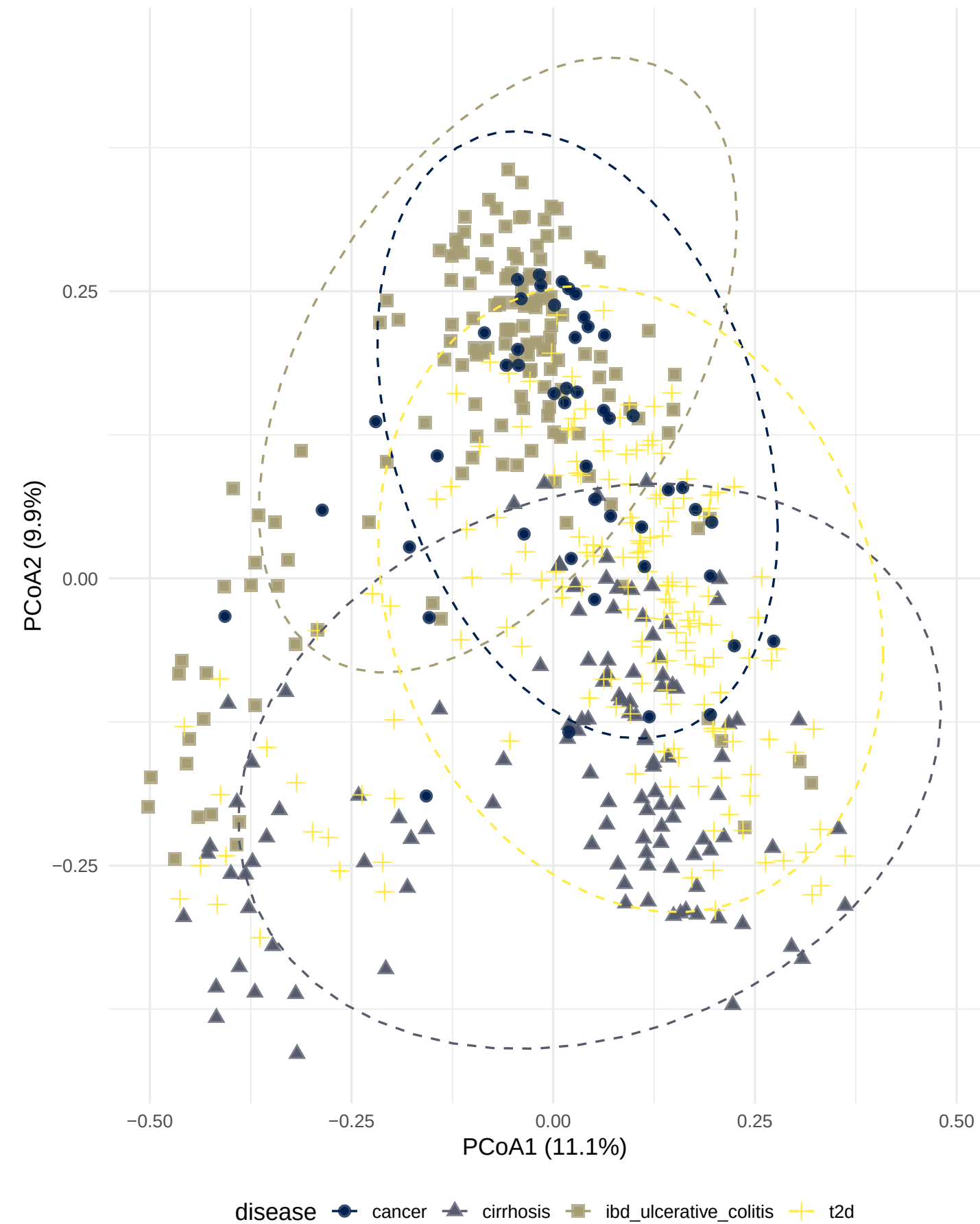
Bray–Curtis Dissimilarity
