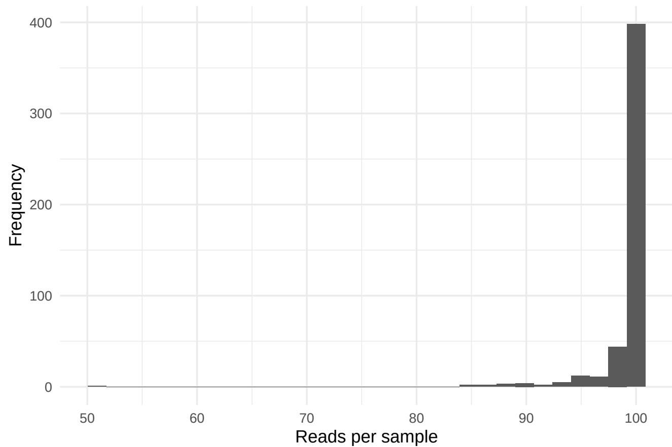
Distribution of Sequencing Depth
