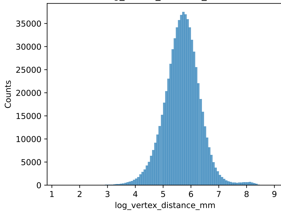
log_vertex_distance_mm
