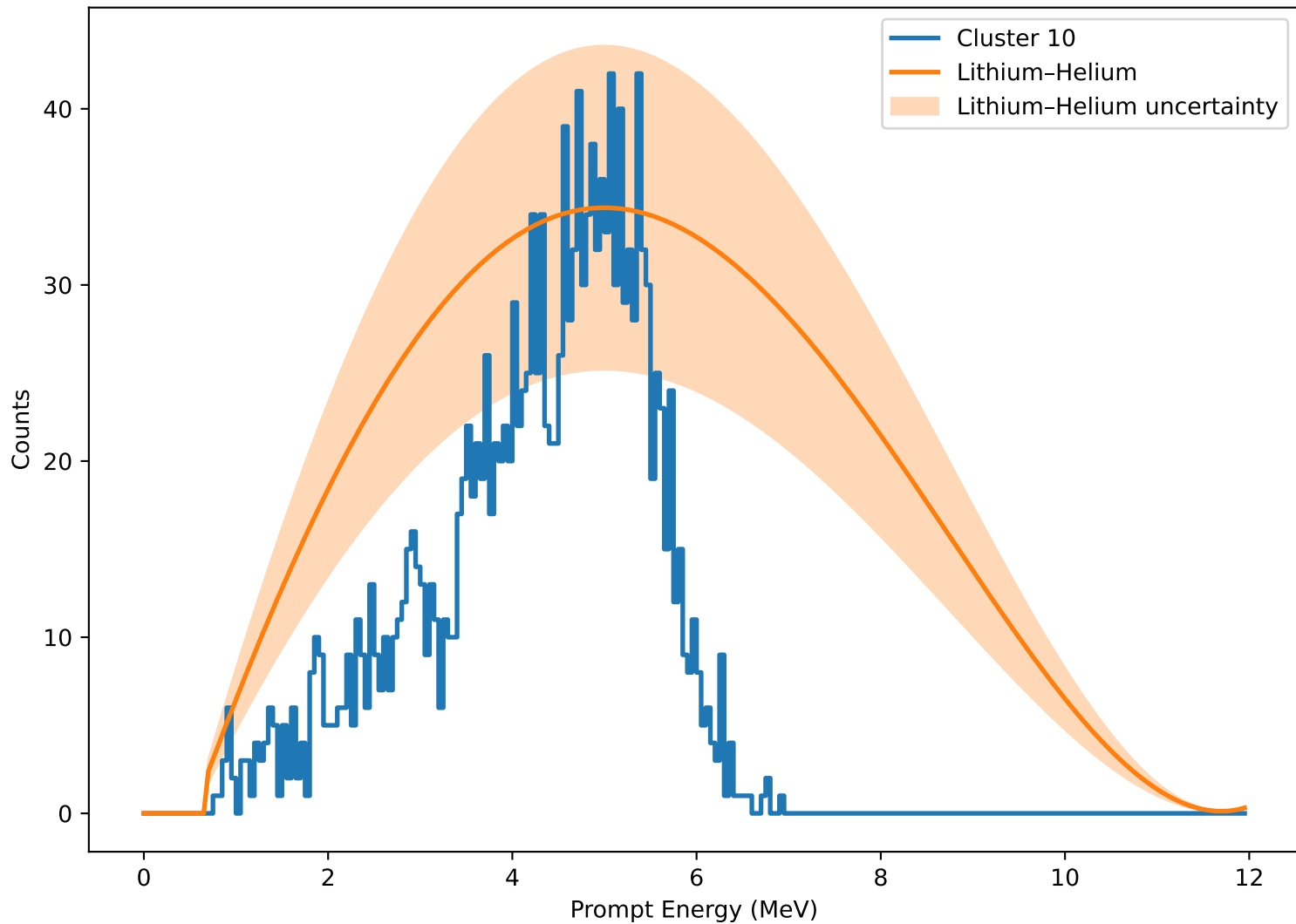
Cluster 10 vs Lithium-Helium Background
