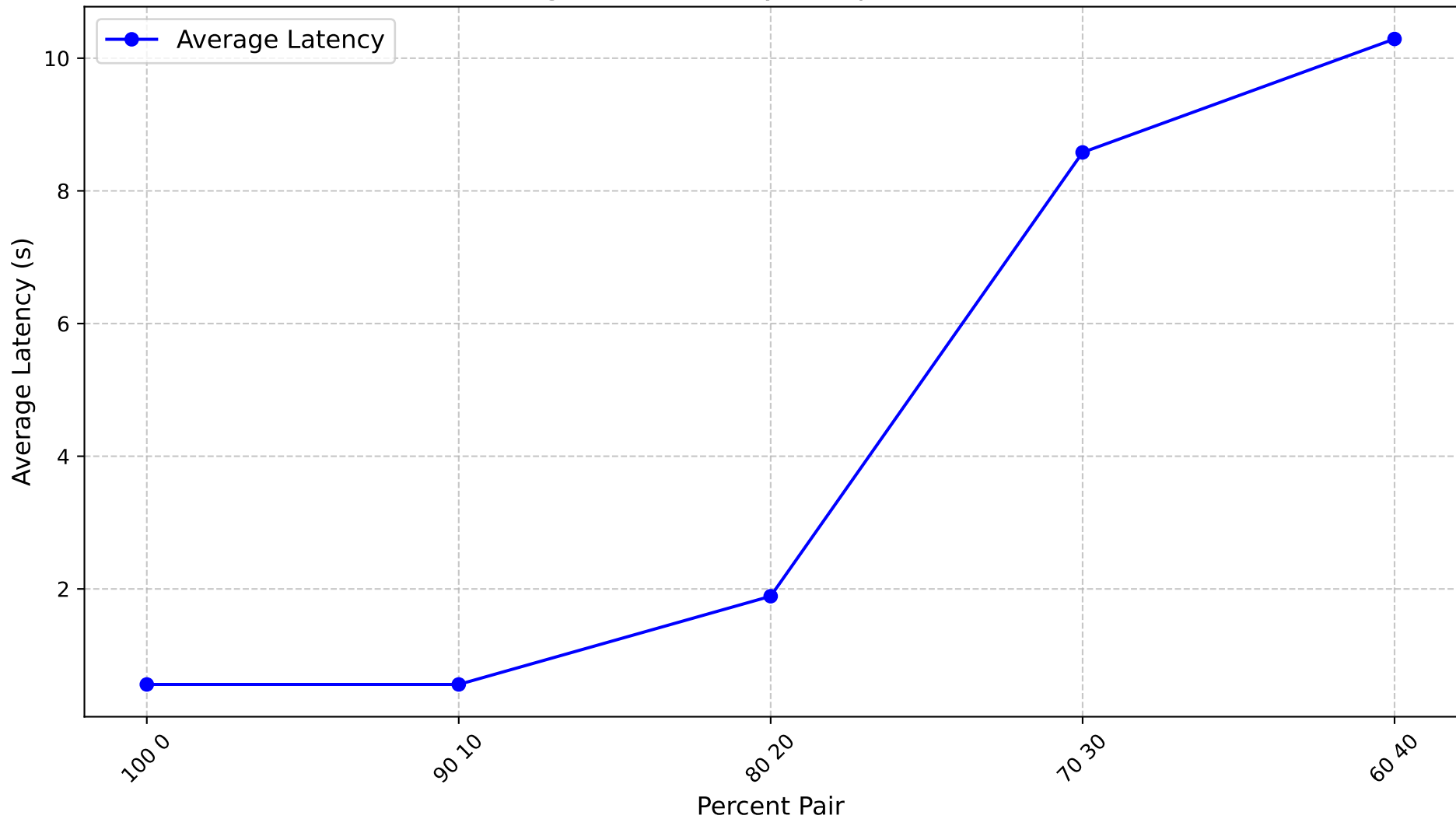
Average Total Latency for opt-6.7b of mine
