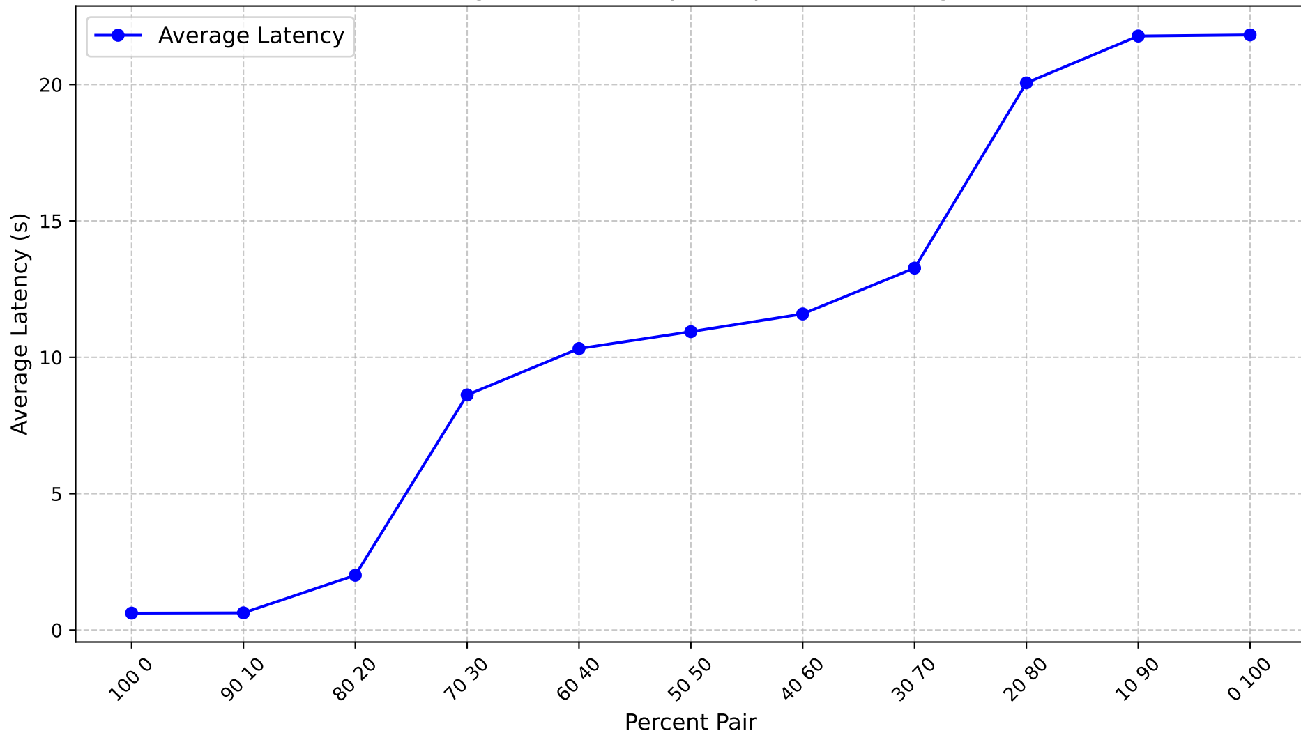
Average Total Latency for opt-6.7b of flexgen
