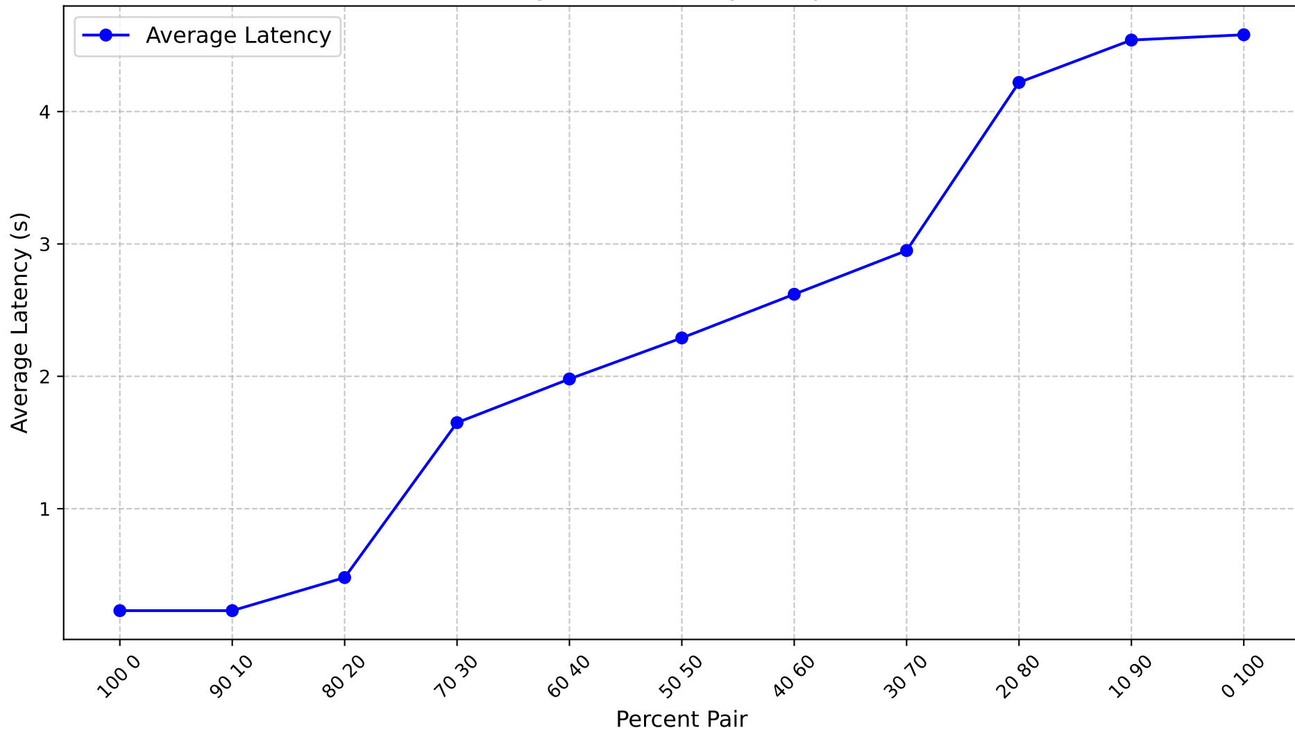
Average Total Latency for opt-1.3b
