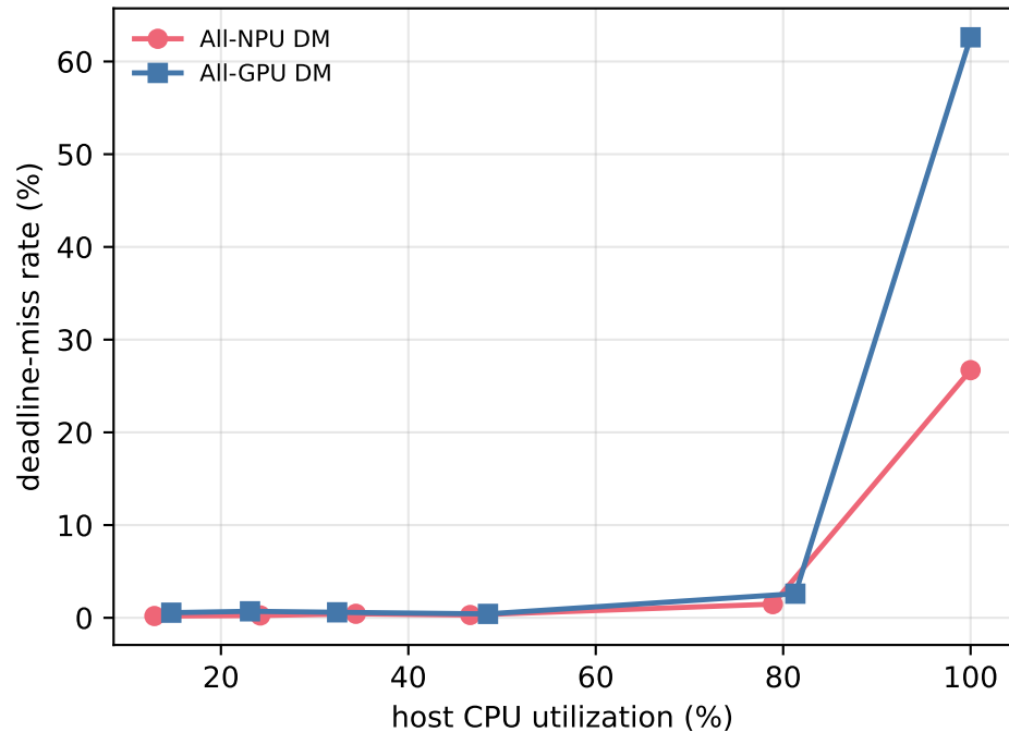
(b) deadline-miss vs host-CPU contention
