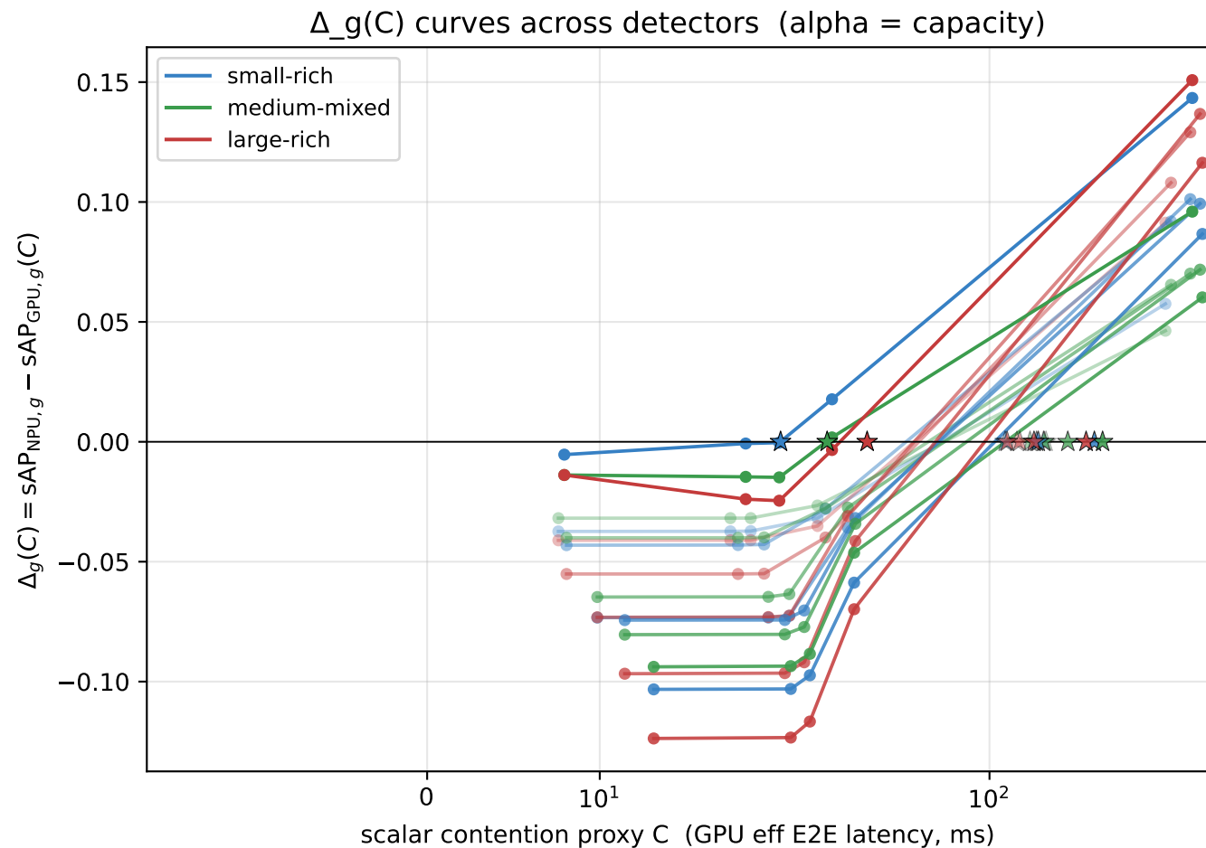
Fig.~gen-cstar — YOLOv8 family + YOLOv11s marker (NEW C* via sAP-gap)
