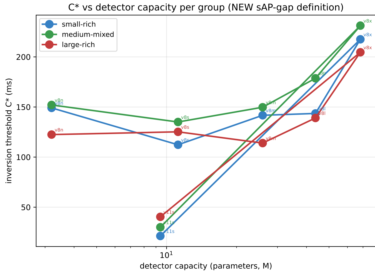
Fig.~gen-cstar — YOLOv8 family + YOLOv11s marker (NEW C* via sAP-gap)
