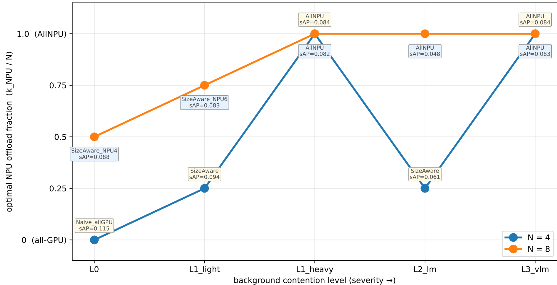
Part B — Optimal offload schedule shifts toward AIINPU under heavier contention
