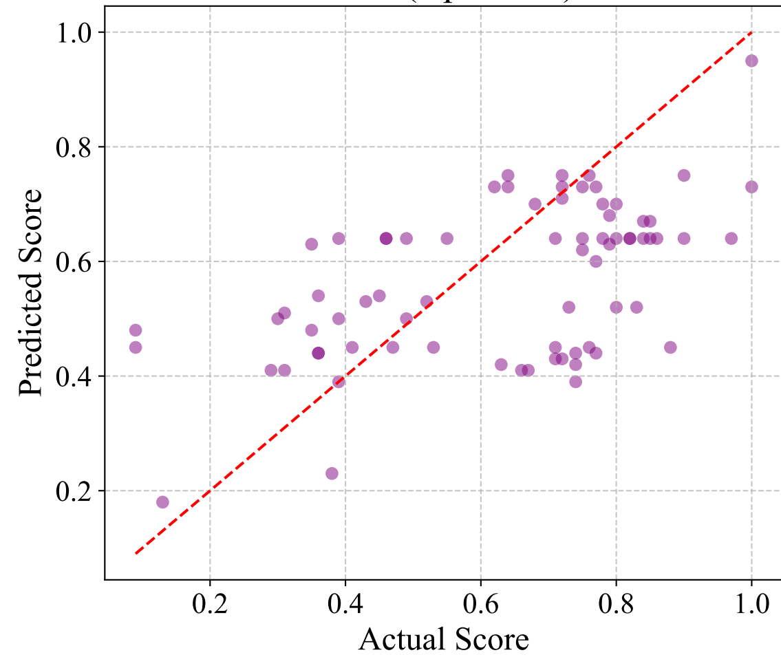
Score (alpha=0.2)
