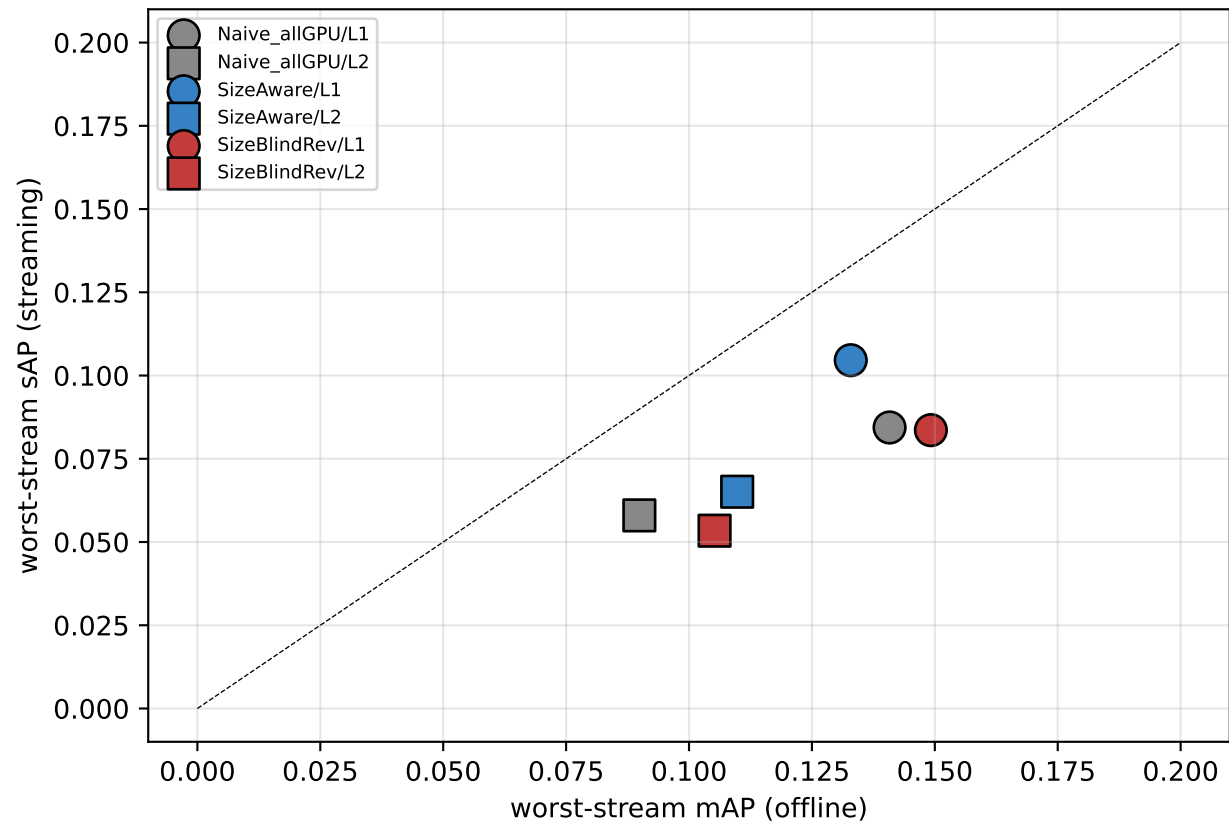
worst-stream sAP vs mAP (distance from y = x = latency penalty)
