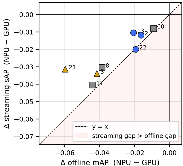
(a) Per-camera quantization gap at L1_{\text{light}} , ordered by NPU loss (b) Offline mAP gap vs streaming sAP gap
