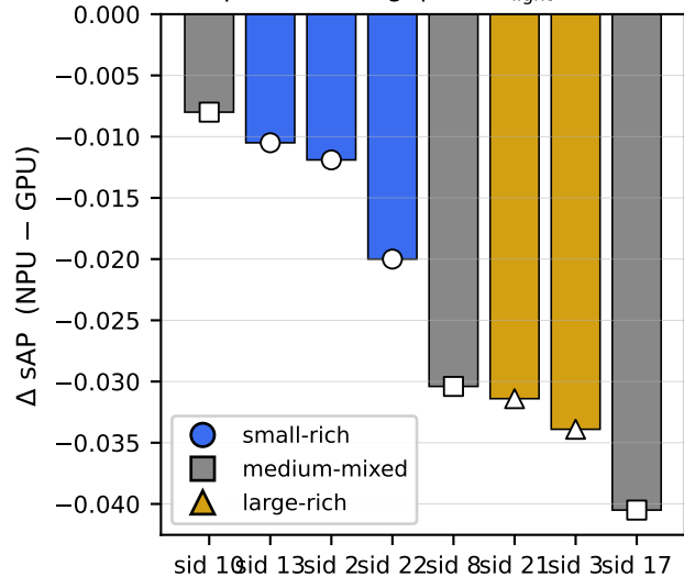
(a) Per-camera quantization gap at L1_{\text{light}} , ordered by NPU loss (b) Offline mAP gap vs streaming sAP gap
