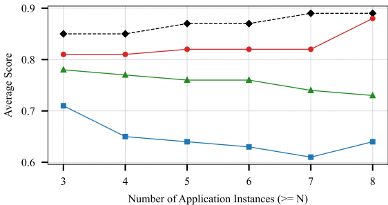
Score vs. Number of Application Instances Legend: Oracle (black dashed line with diamonds), Ours (red solid line with circles), Best-of-5 (green solid line with triangles), Latency-based (blue solid line with squares).
