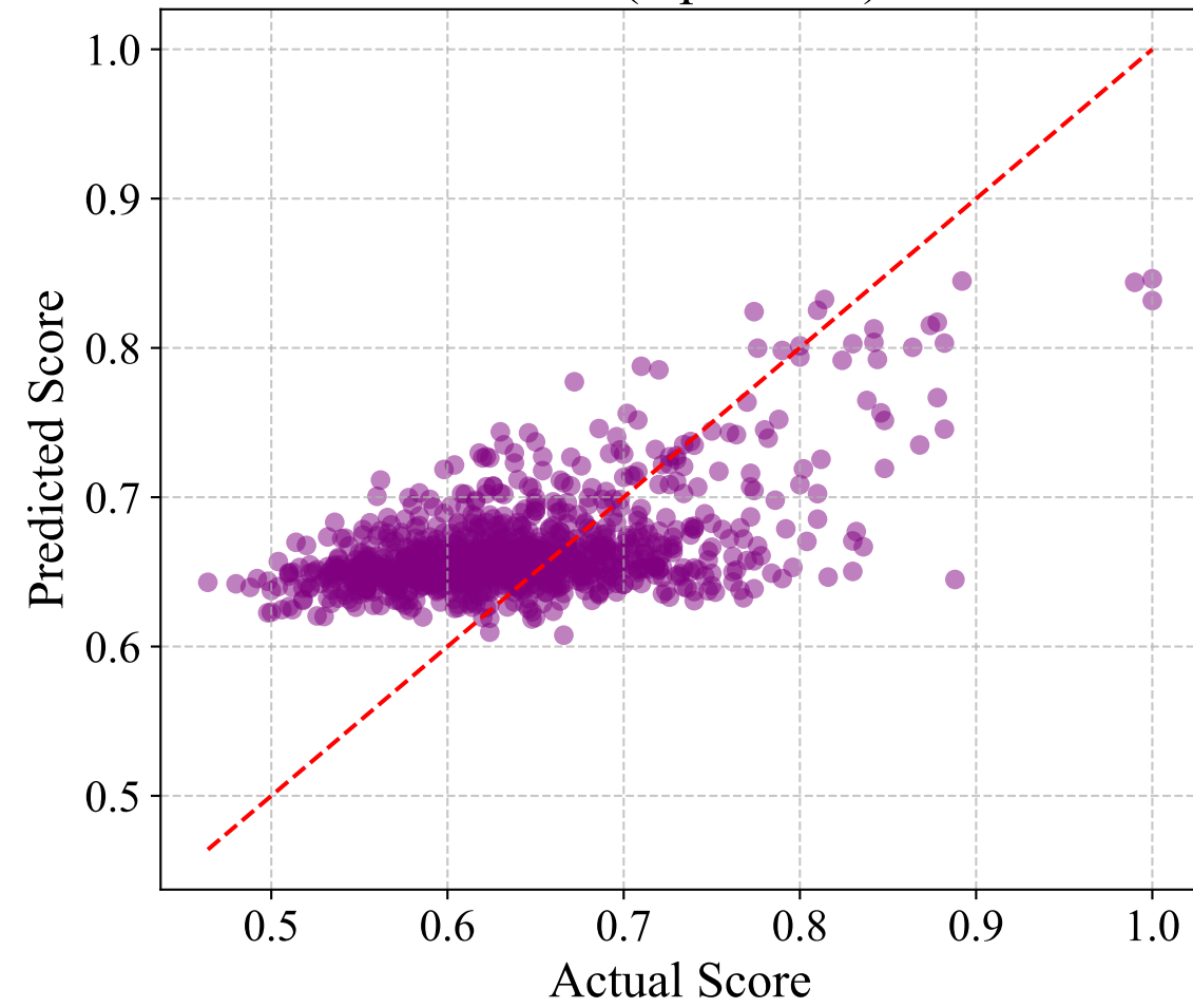
Score (alpha=0.2)
