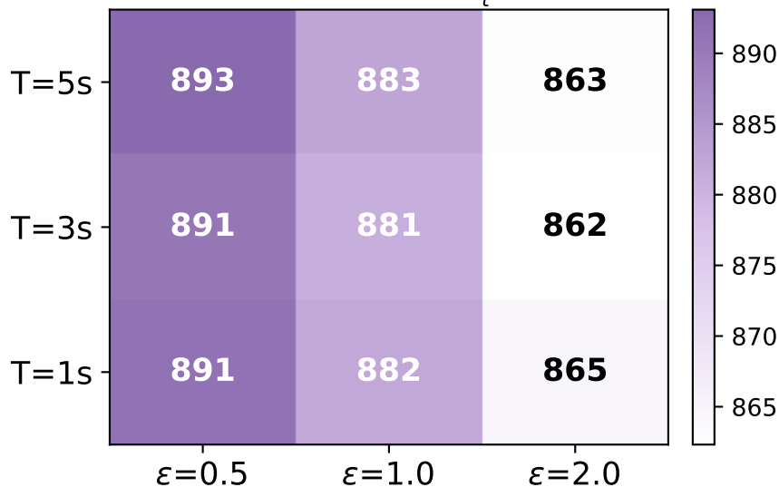
Cumulative violation \sum_t (V(t) - \epsilon)^+
