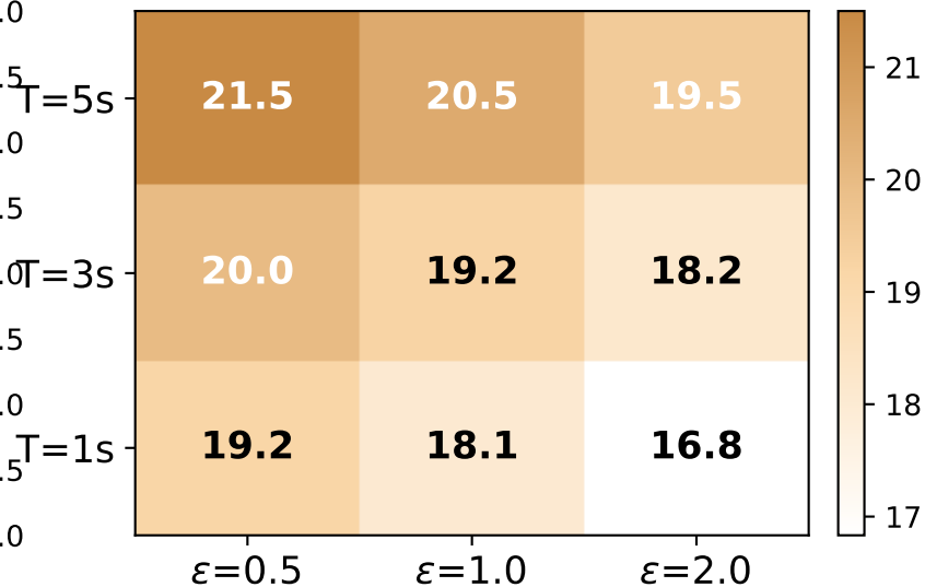
Cumulative violation \sum_t (V(t) - \epsilon)^+
