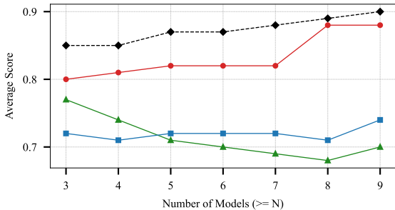
Score vs. Number of Models Legend: Oracle (black dashed line with diamond markers), Ours (red solid line with circle markers), Best-of-5 (green solid line with triangle markers), Latency-based (blue solid line with square markers).
