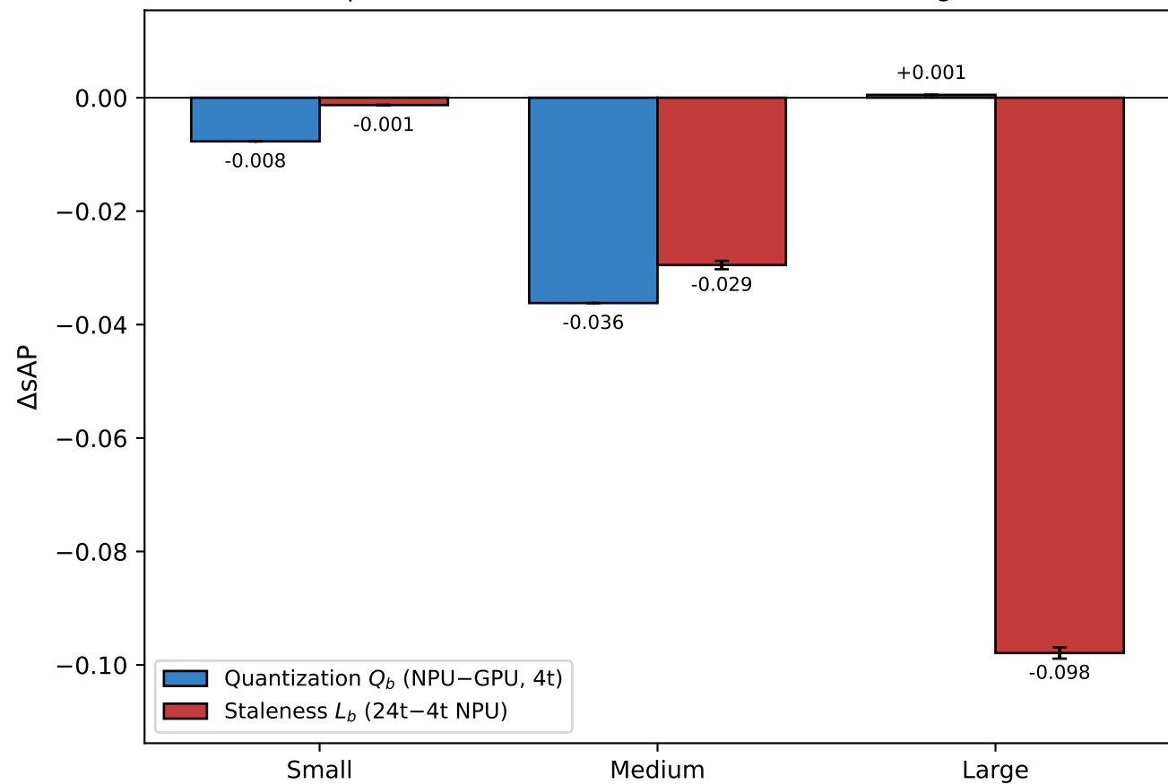
Per-size quantization vs staleness loss (YOLOv11s, single stream)
