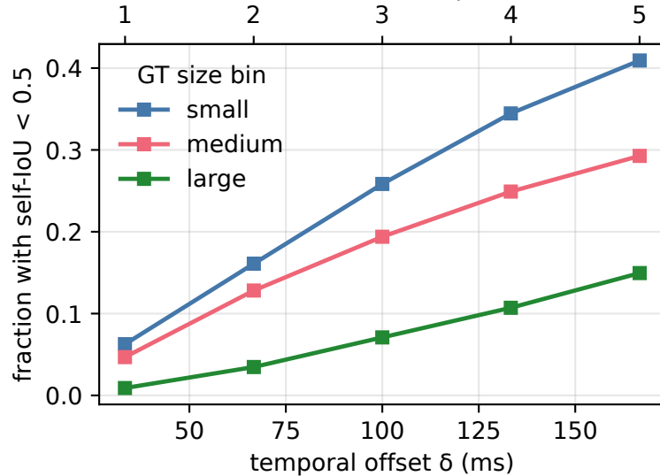
(b) Fraction below COCO match threshold
