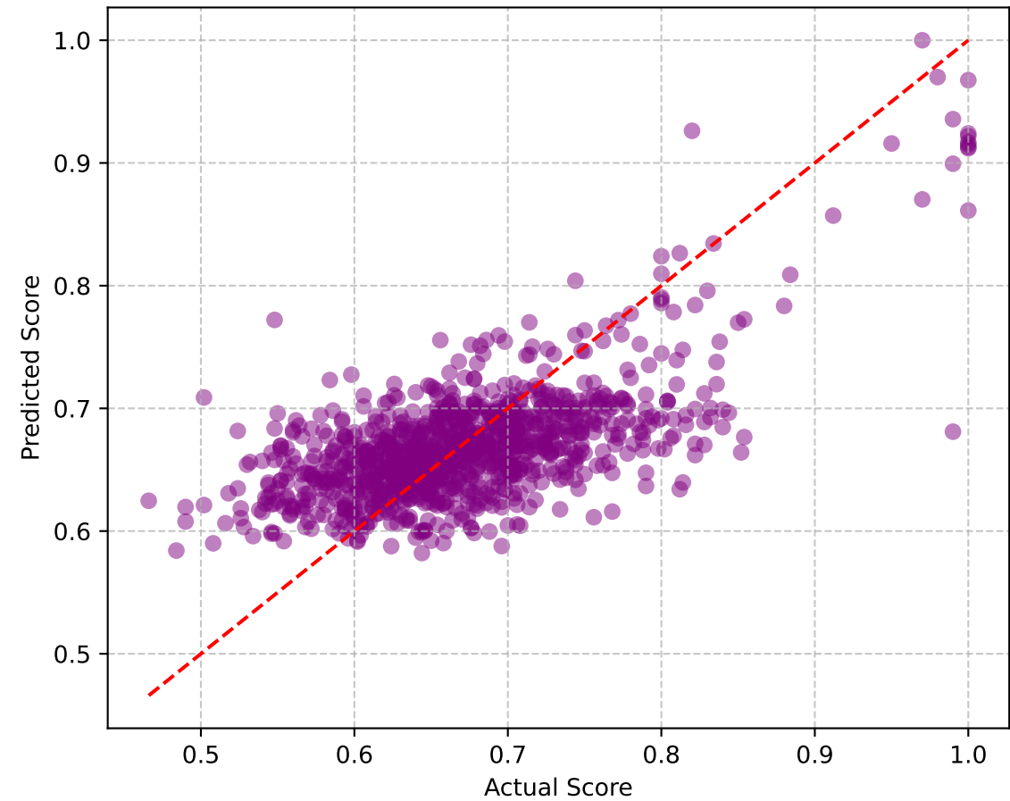
Combined Score (alpha=0.2)
