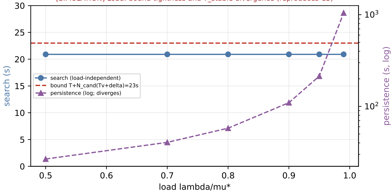
[SIMULATION] Load: bound tightness and T_stable divergence (reproduces C3)
