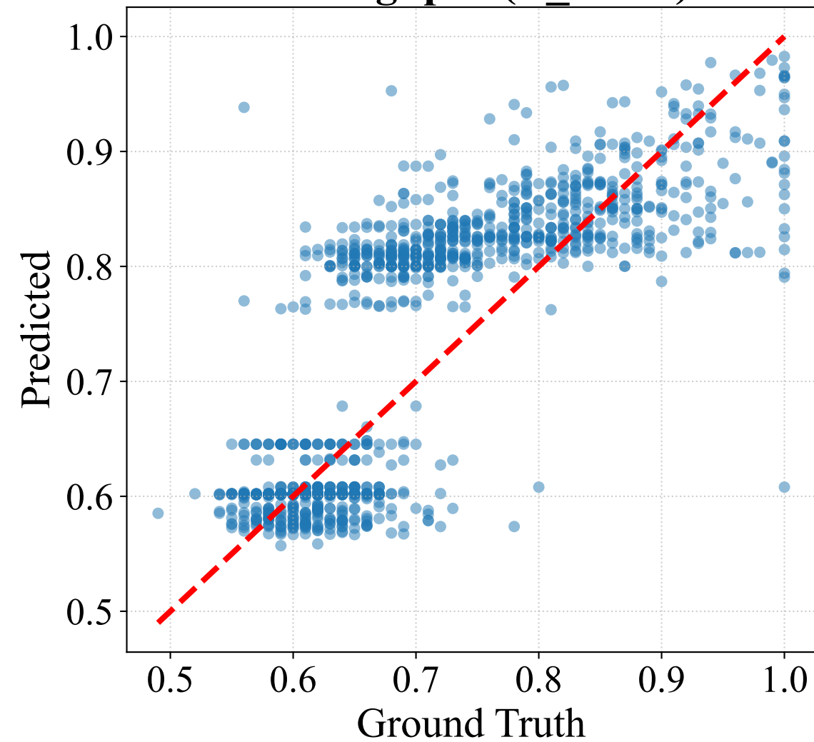
Throughput (T_norm)
