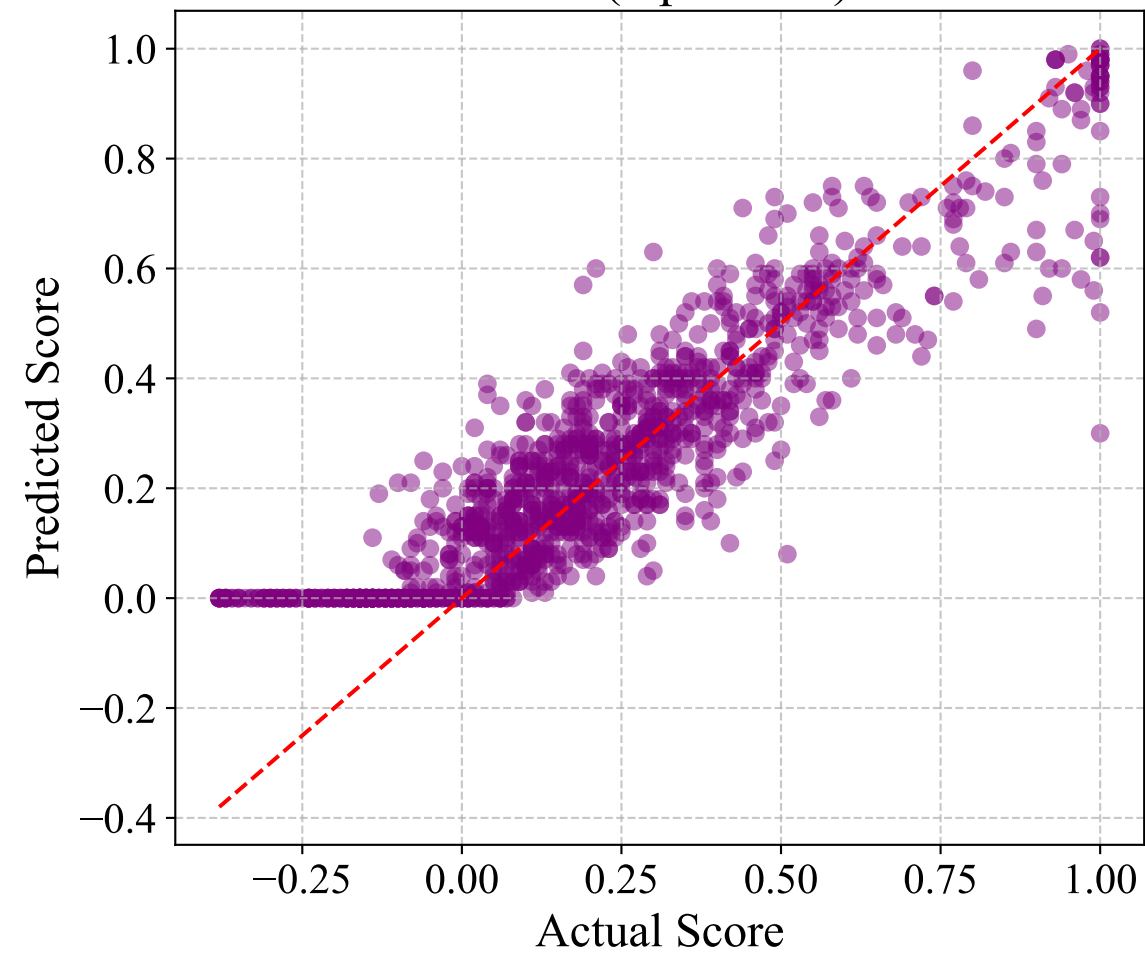
Score (alpha=0.4)
