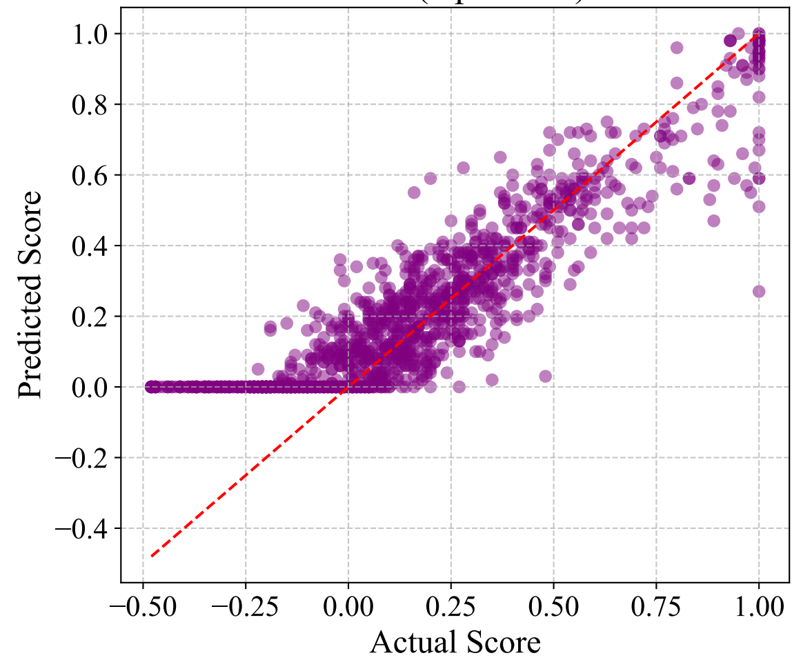
Score (alpha=0.5)
