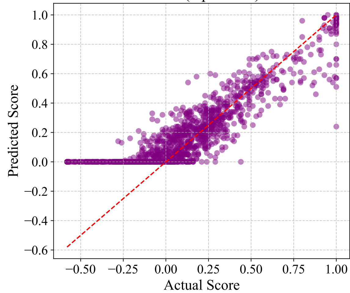
Score (alpha=0.6)
