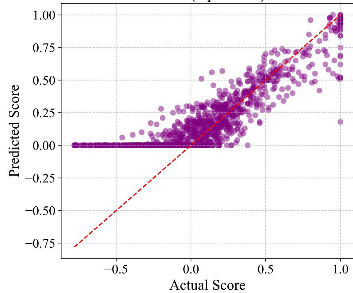
Score (alpha=0.8)
