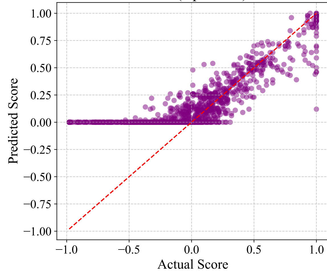
Score (alpha=1.0)
