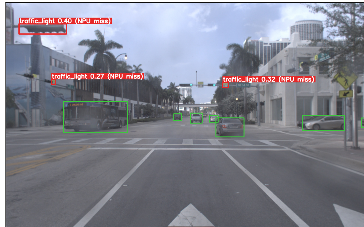
sid 13, frame 41 — NPU misses: traffic_light, traffic_light, traffic_light
