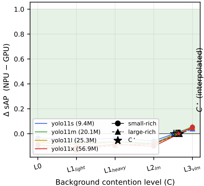
(a) Per-detector device-gap across bg ladder
