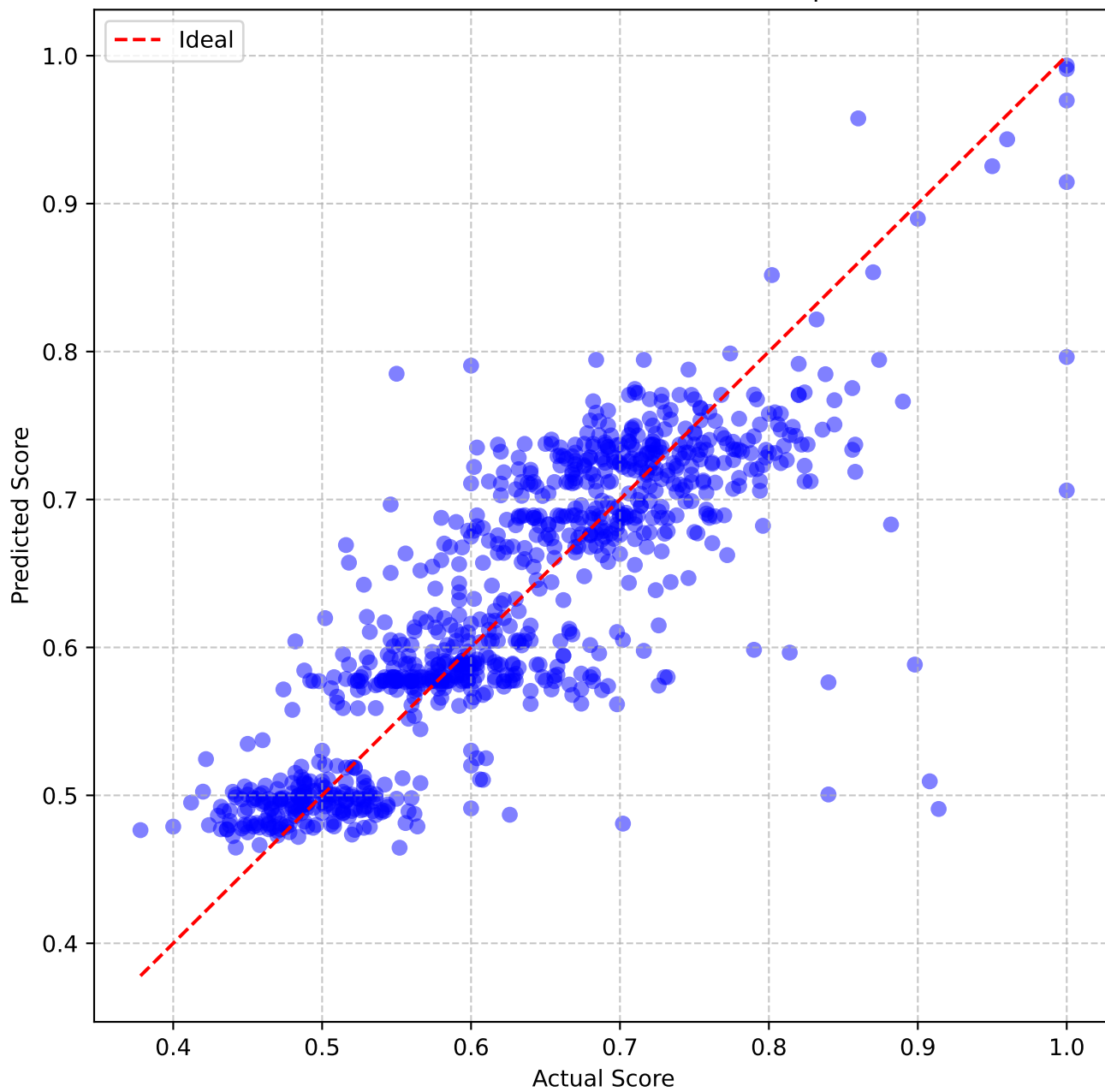
Score Prediction: Actual vs Predicted (alpha=0.2)
