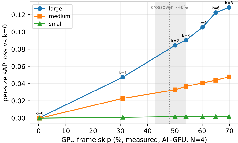
Per-size sAP loss vs GPU contention (ResNet50 k-sweep) All-NPU loss \approx 0 (flat, not shown); rerun w/ util sampler
