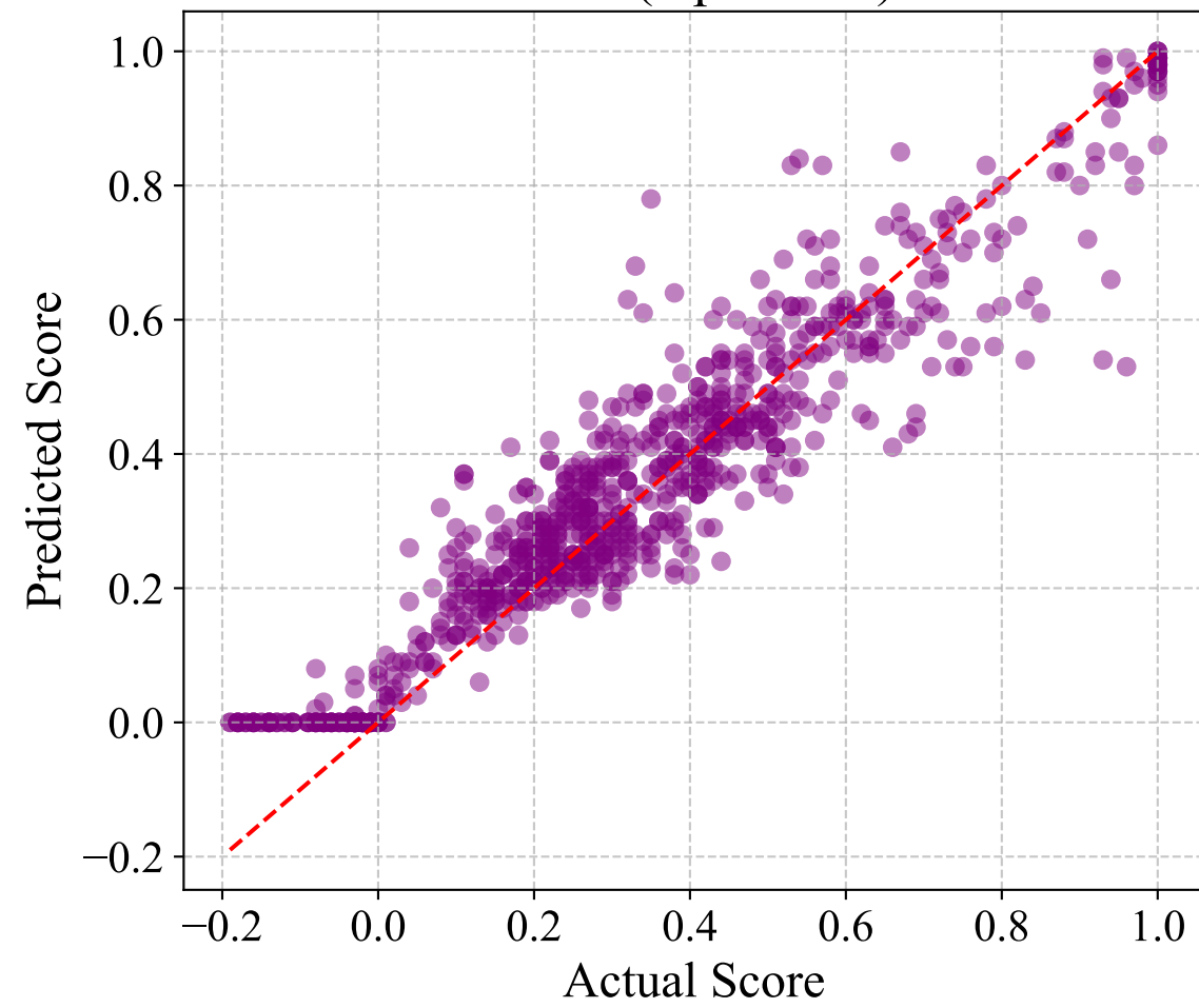
Score (alpha=0.2)
