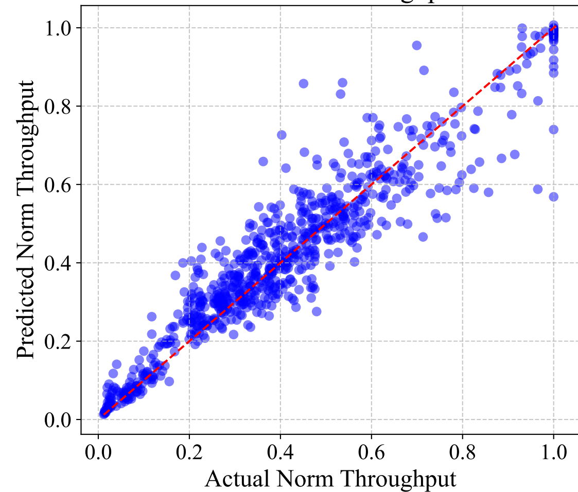
Normalized Throughput
