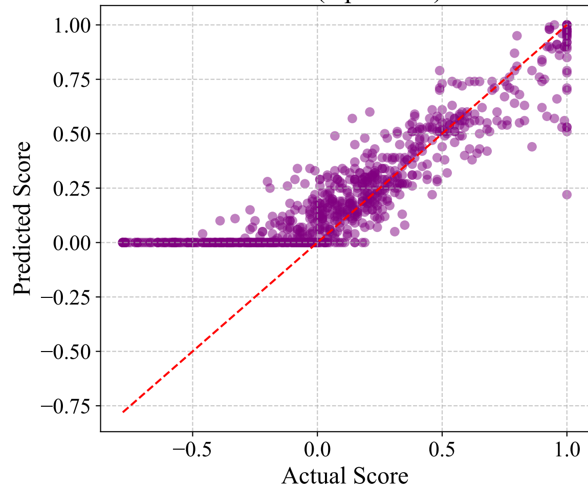
Score (alpha=0.8)
