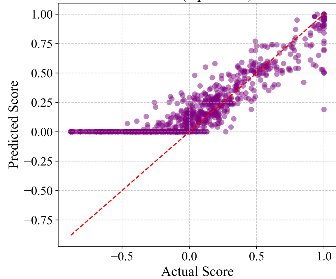
Score (alpha=0.9)
