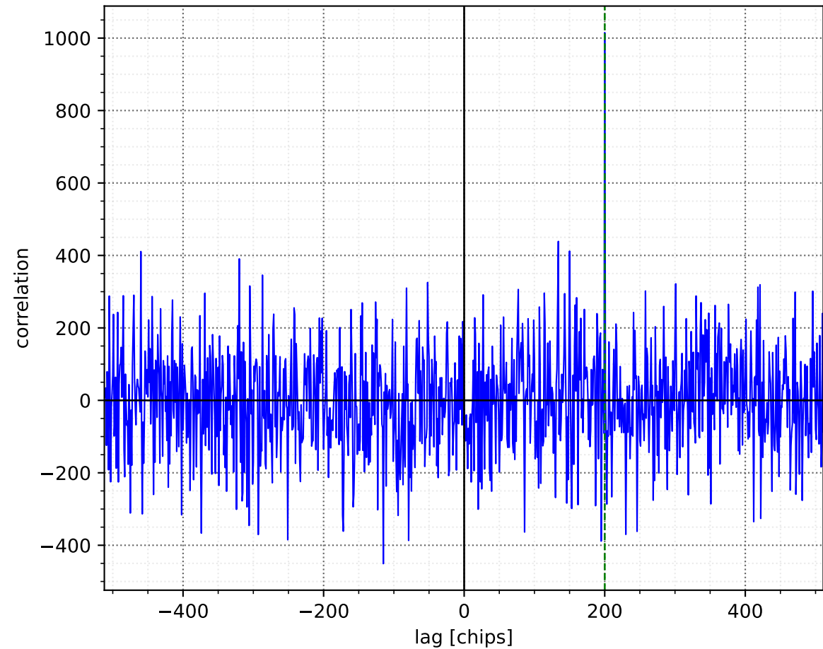
1 period: gain \approx 30 dB
