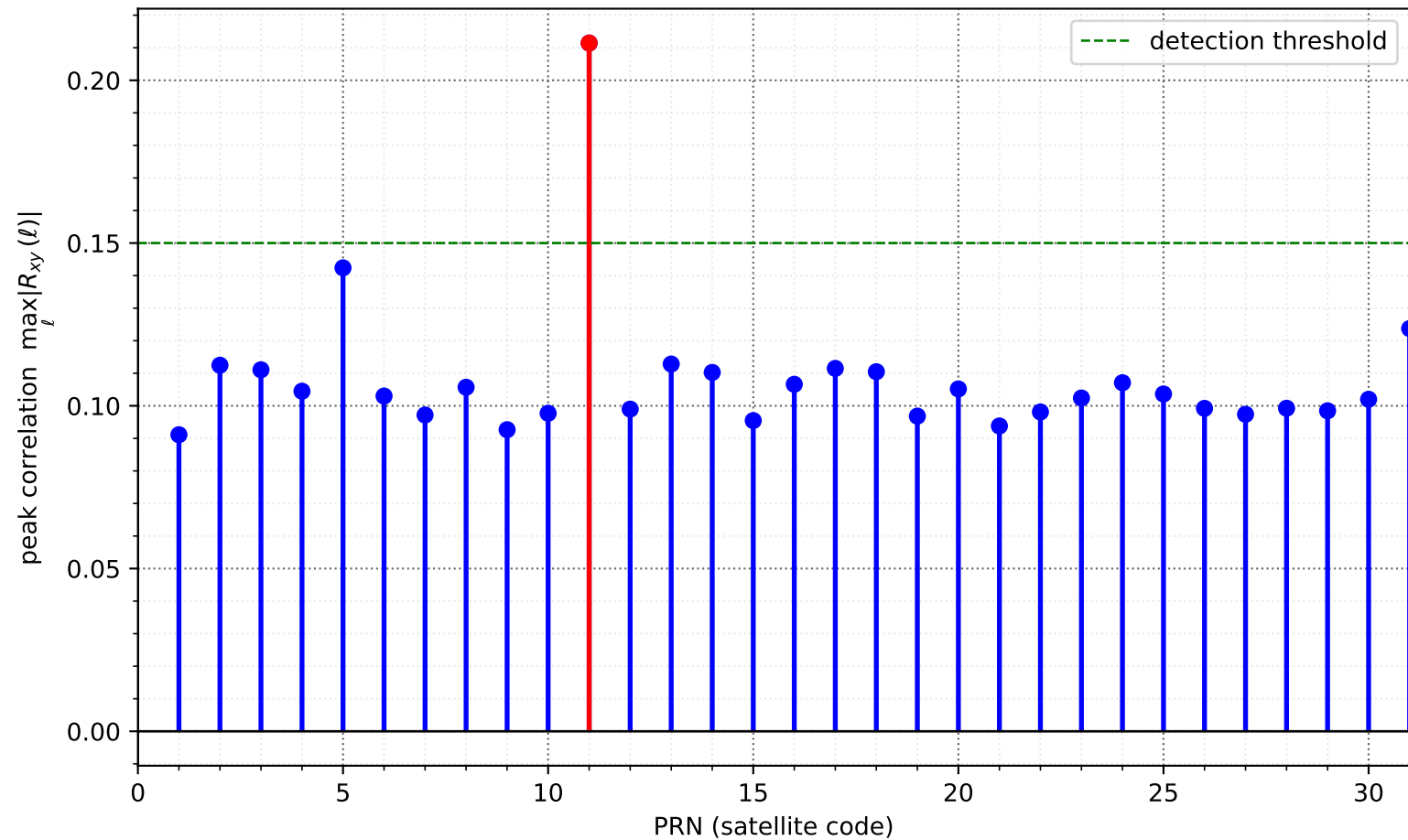
Acquisition: peak correlation per satellite (detected PRN 11)
