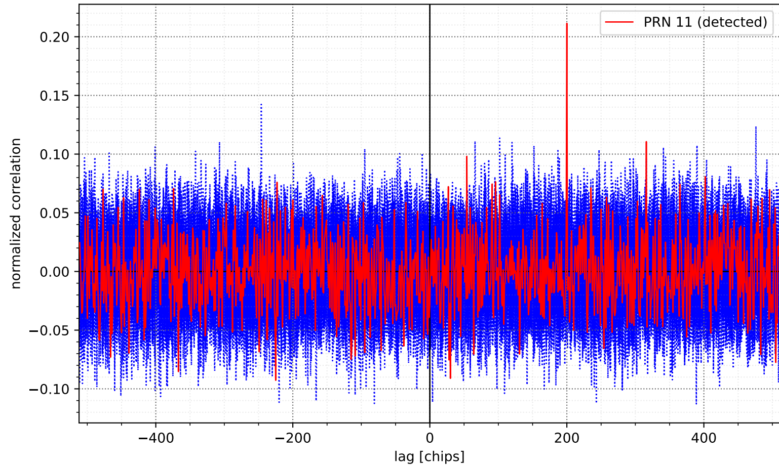
GPS acquisition: scan every PRN, only the present satellite pops out
