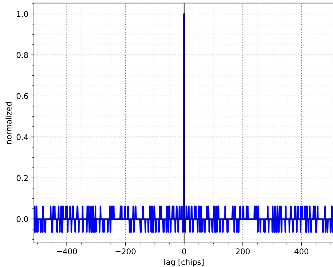
PRN code autocorrelation
