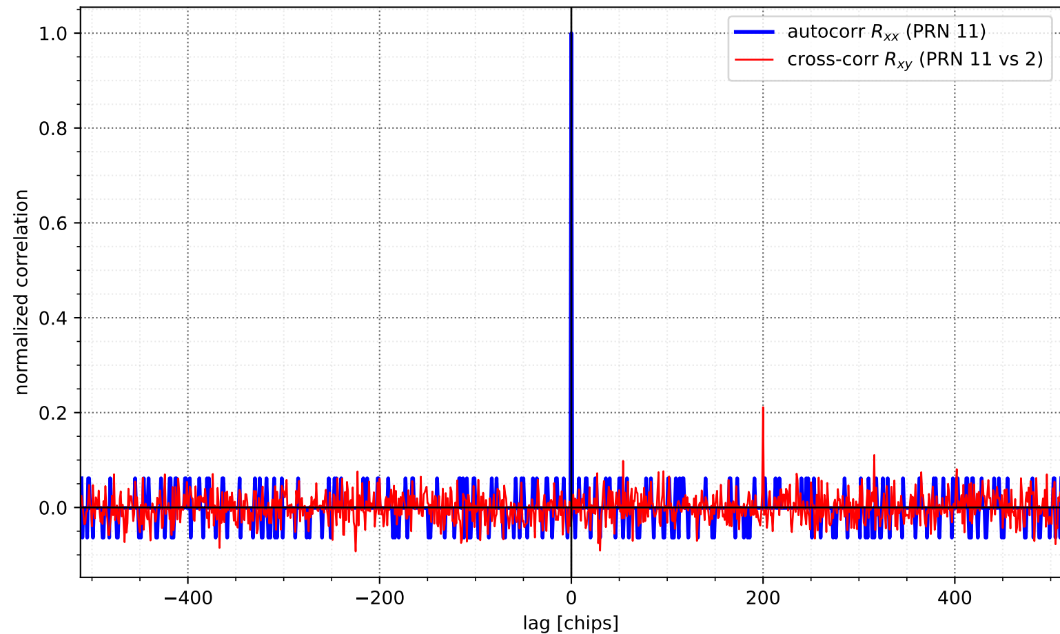
Autocorrelation spike vs near-zero cross-correlation (CDMA)
