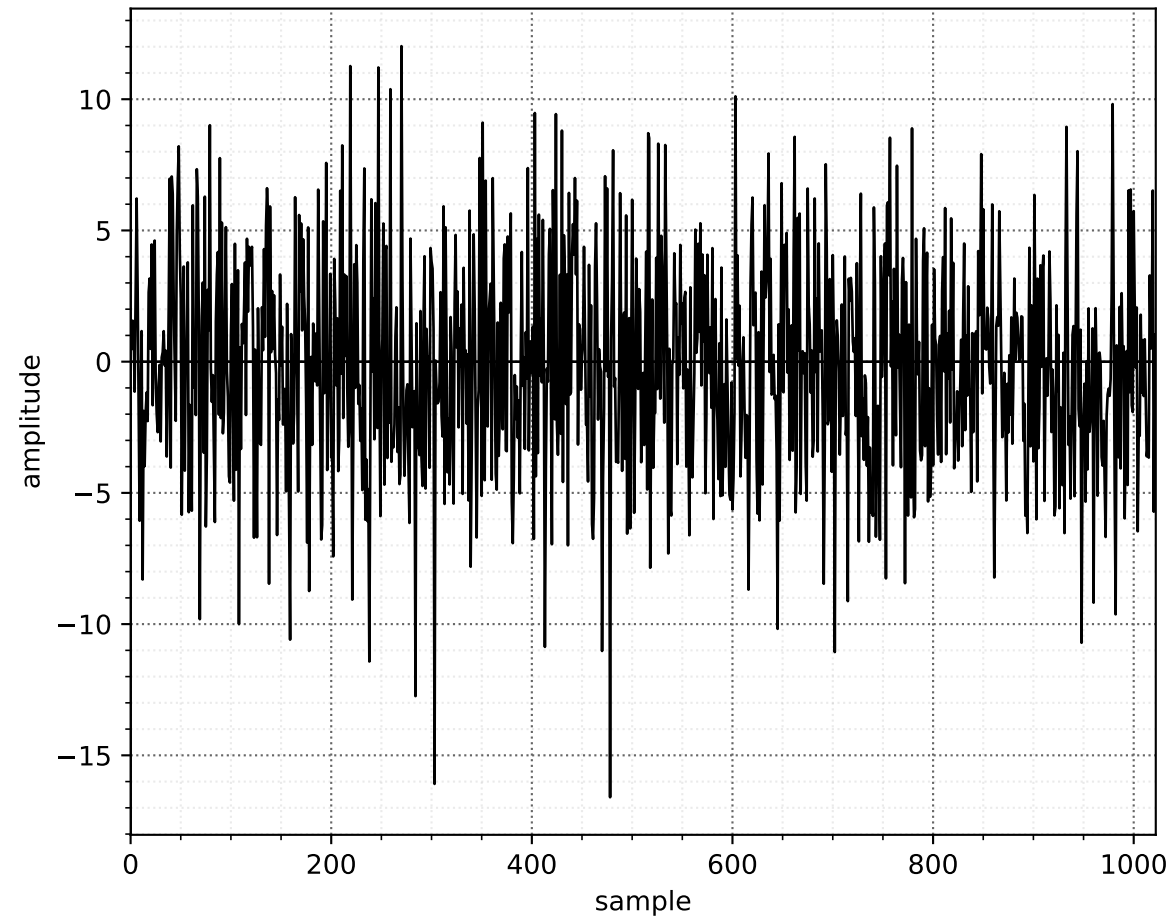
Received: code buried in noise (SNR = -12 dB)
