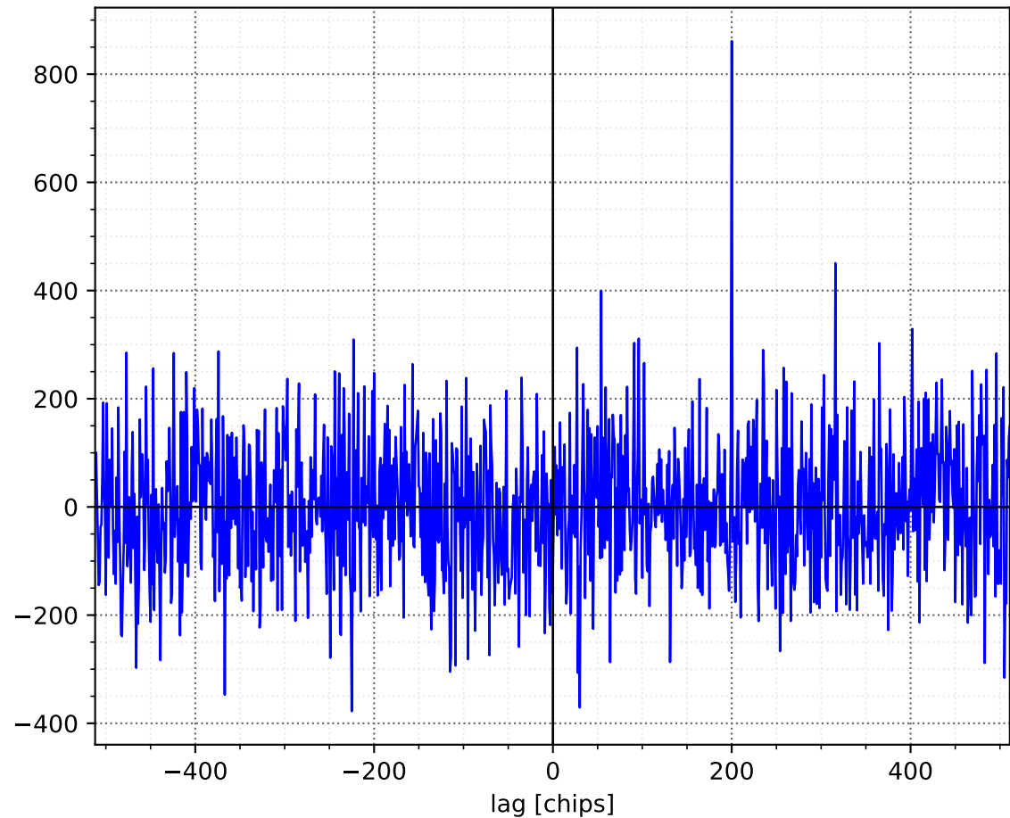
Correlation with replica (gain \approx 30 dB)
