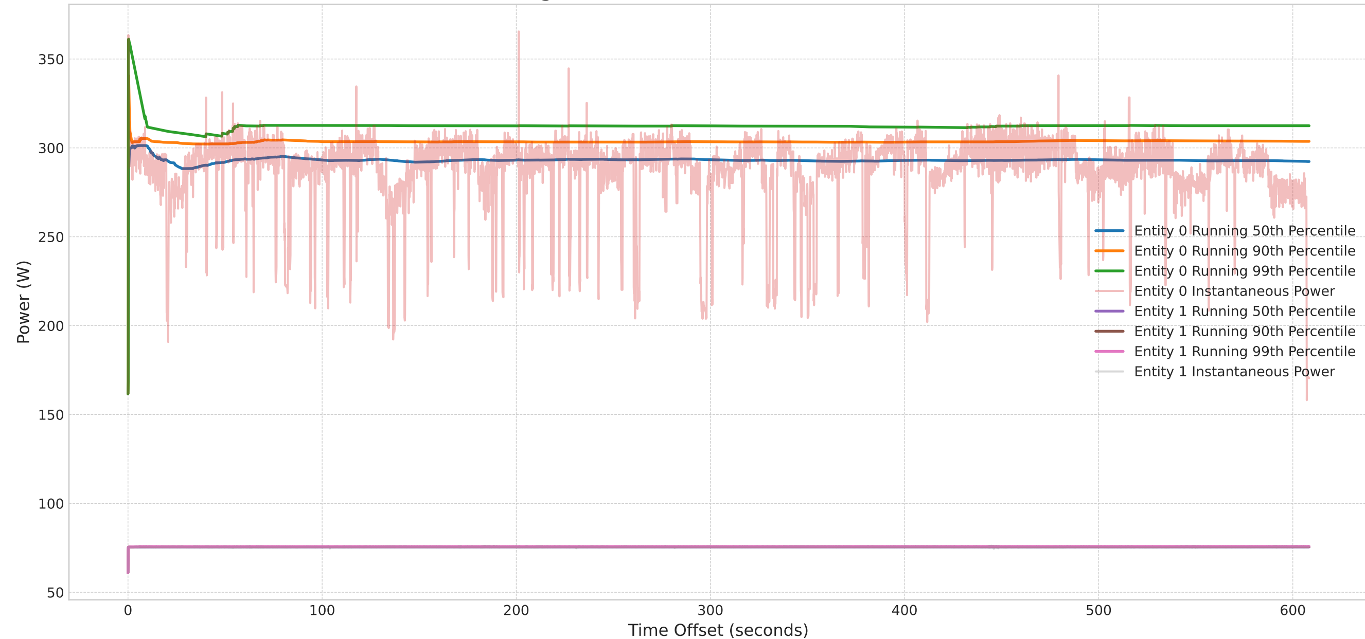
Running Percentiles of Power for Entities [0, 1]
