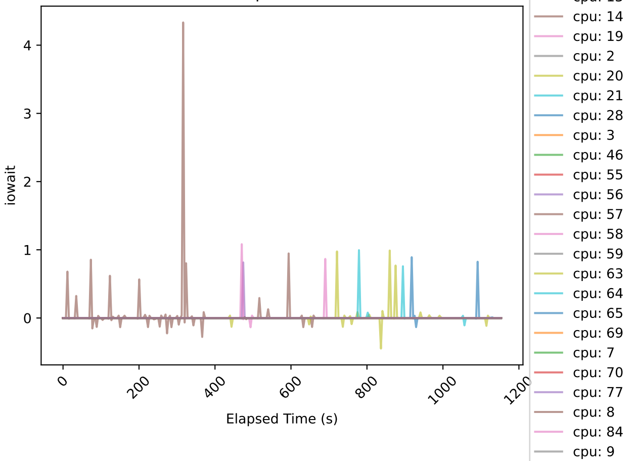
Traces of iowait for each cpu with utilization reaches 100%
