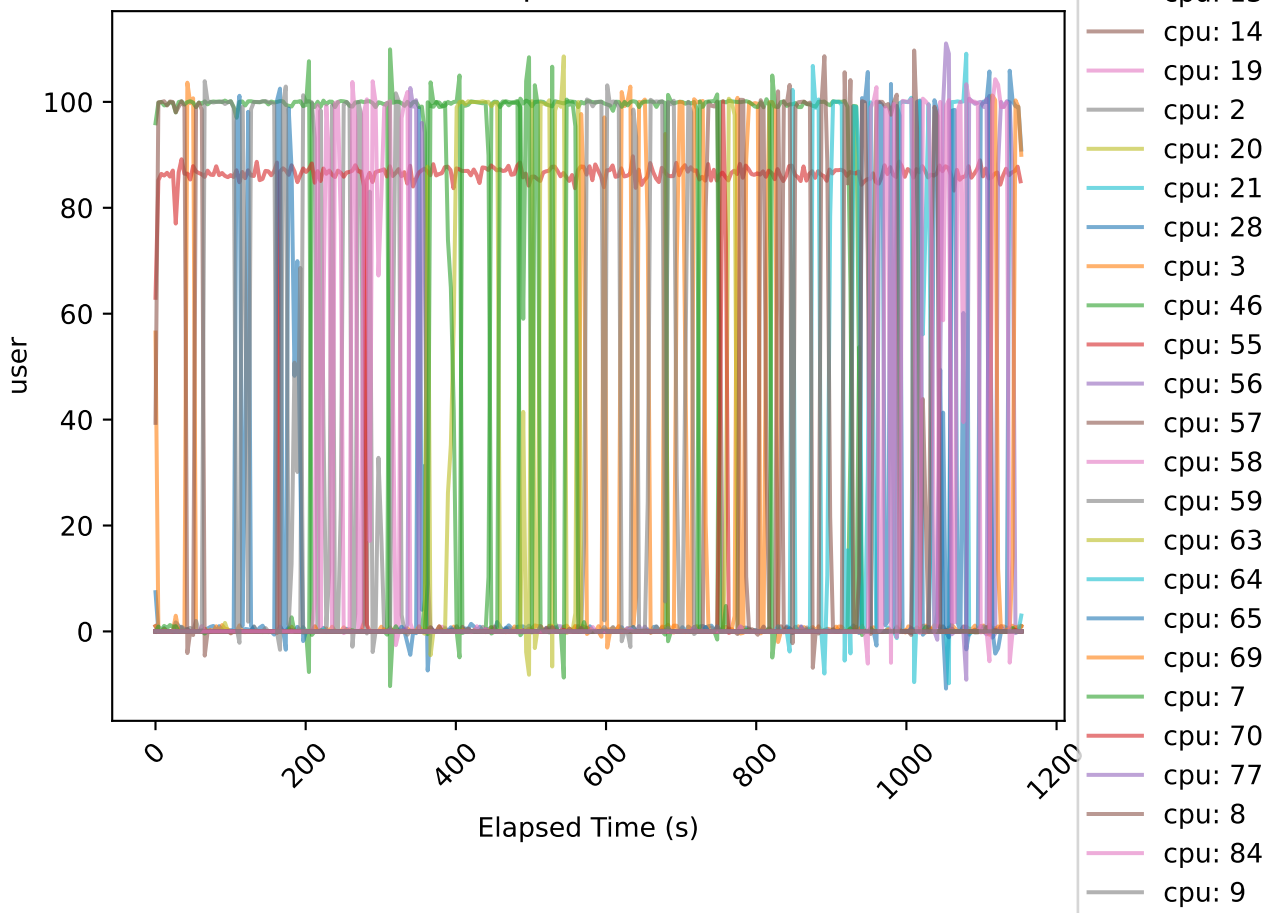
Traces of user for each cpu with utilization reaches 100%
