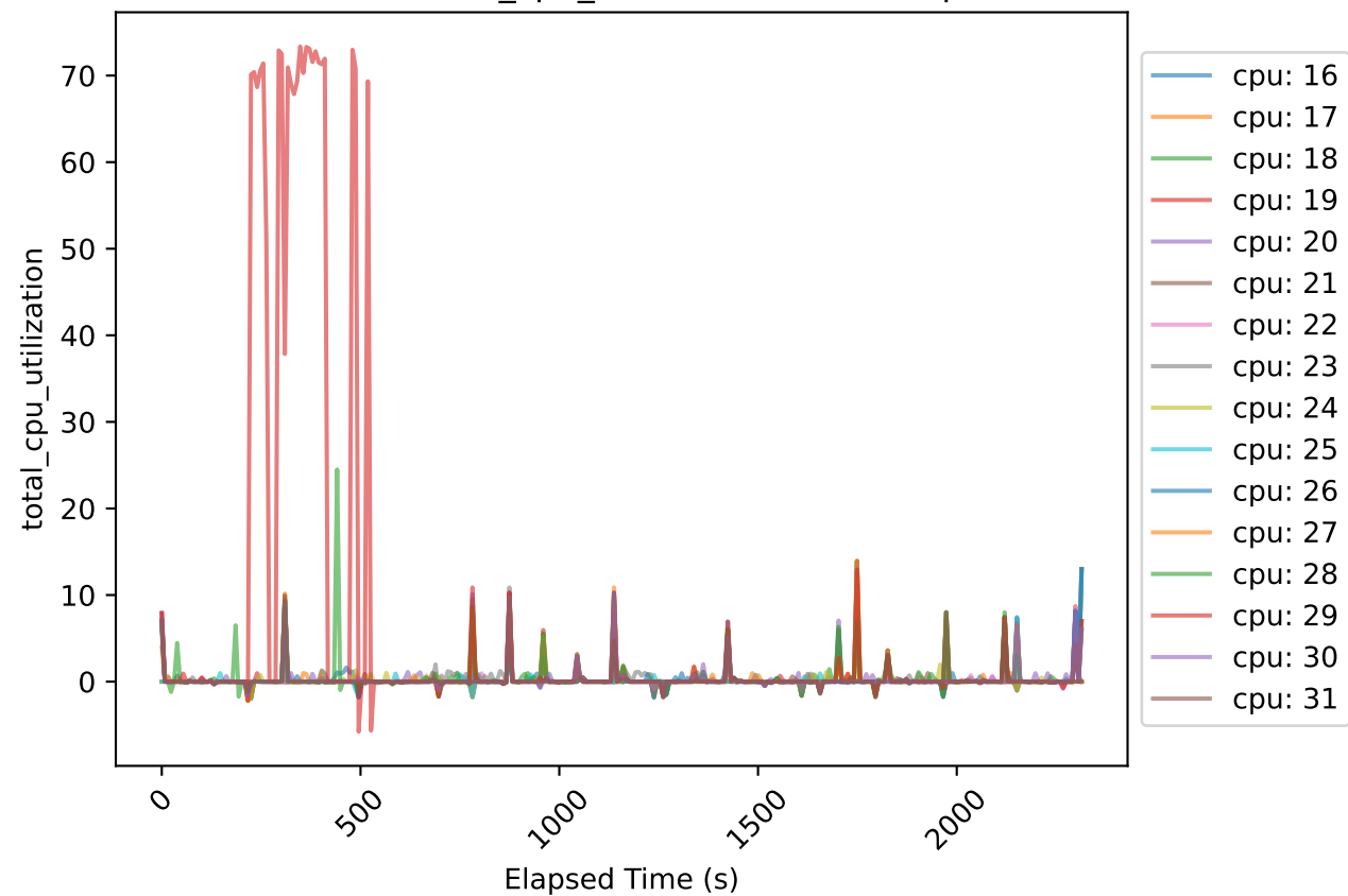
Traces of total cpu utilization for each cpu
