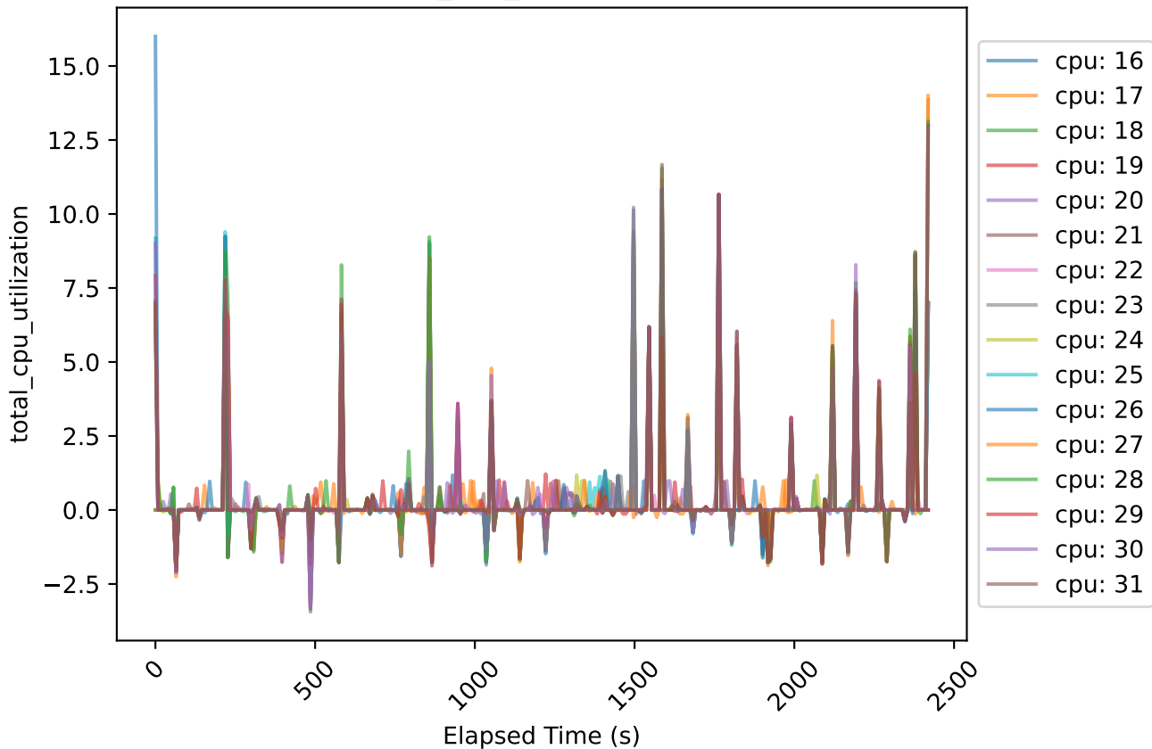
Traces of total cpu utilization for each cpu
