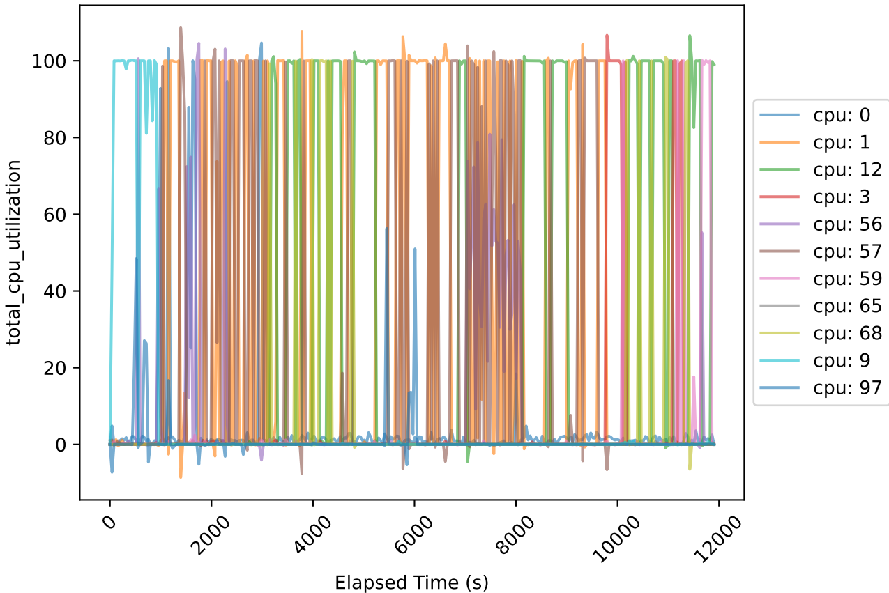
Traces of total_cpu_utilization for each cpu with utilization reaches 100%
