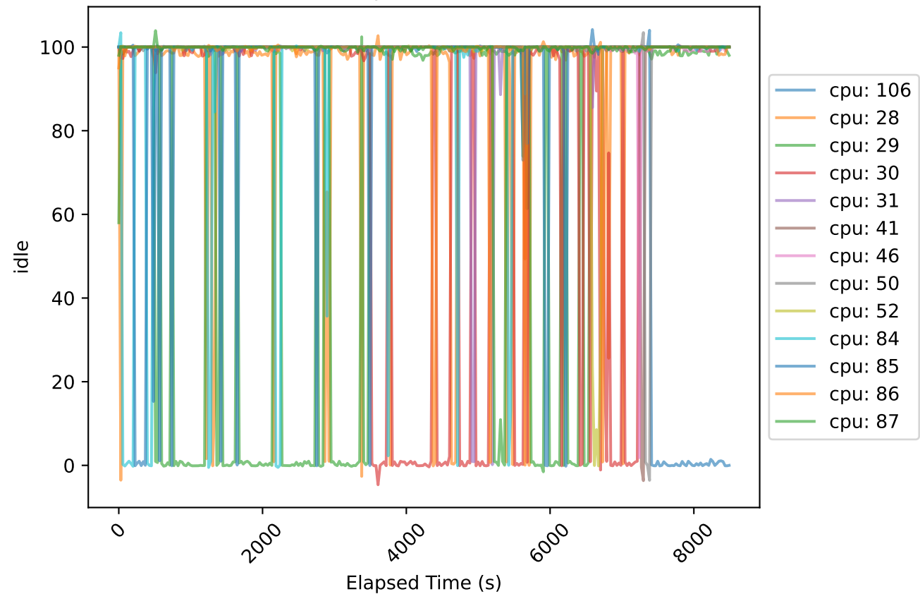
Traces of idle for each cpu with utilization reaches 100%
