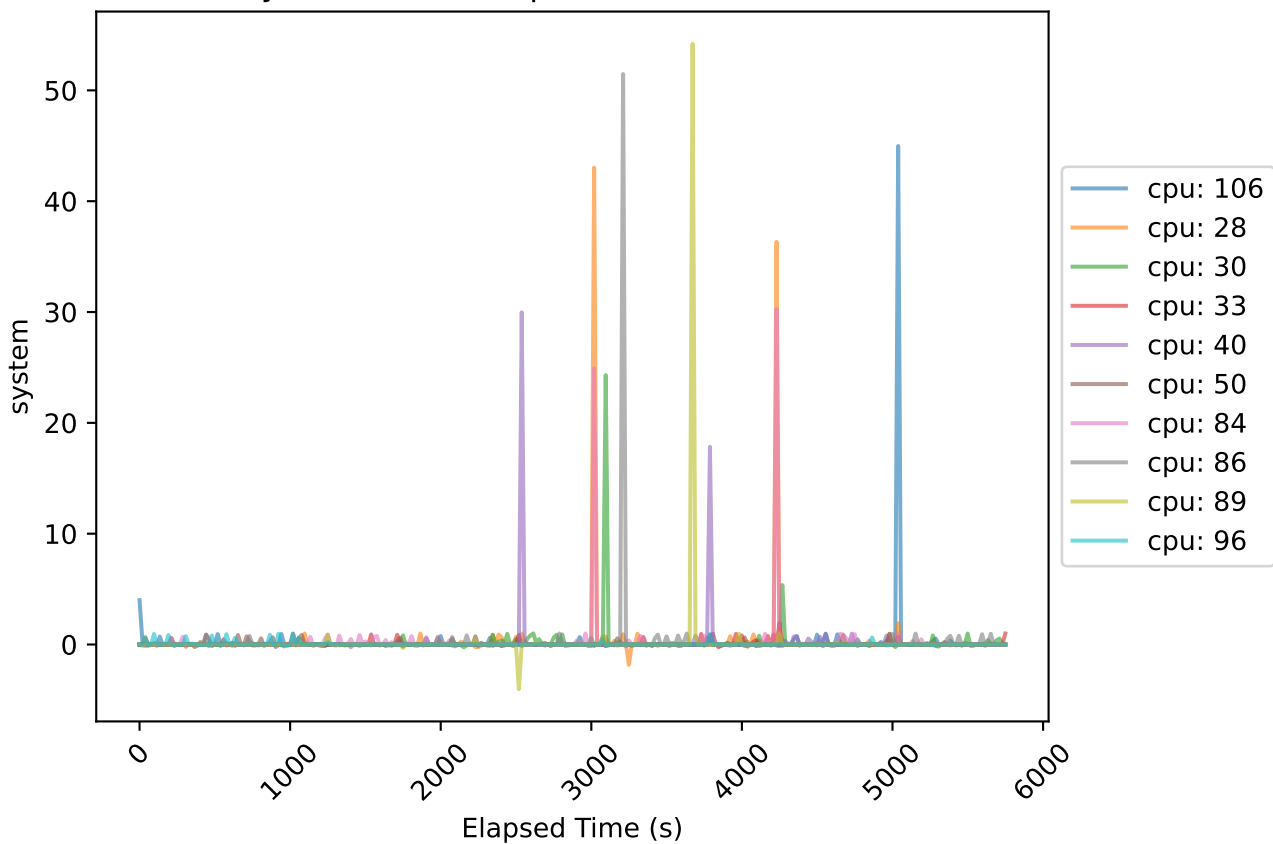
Traces of system for each cpu with utilization reaches 100%
