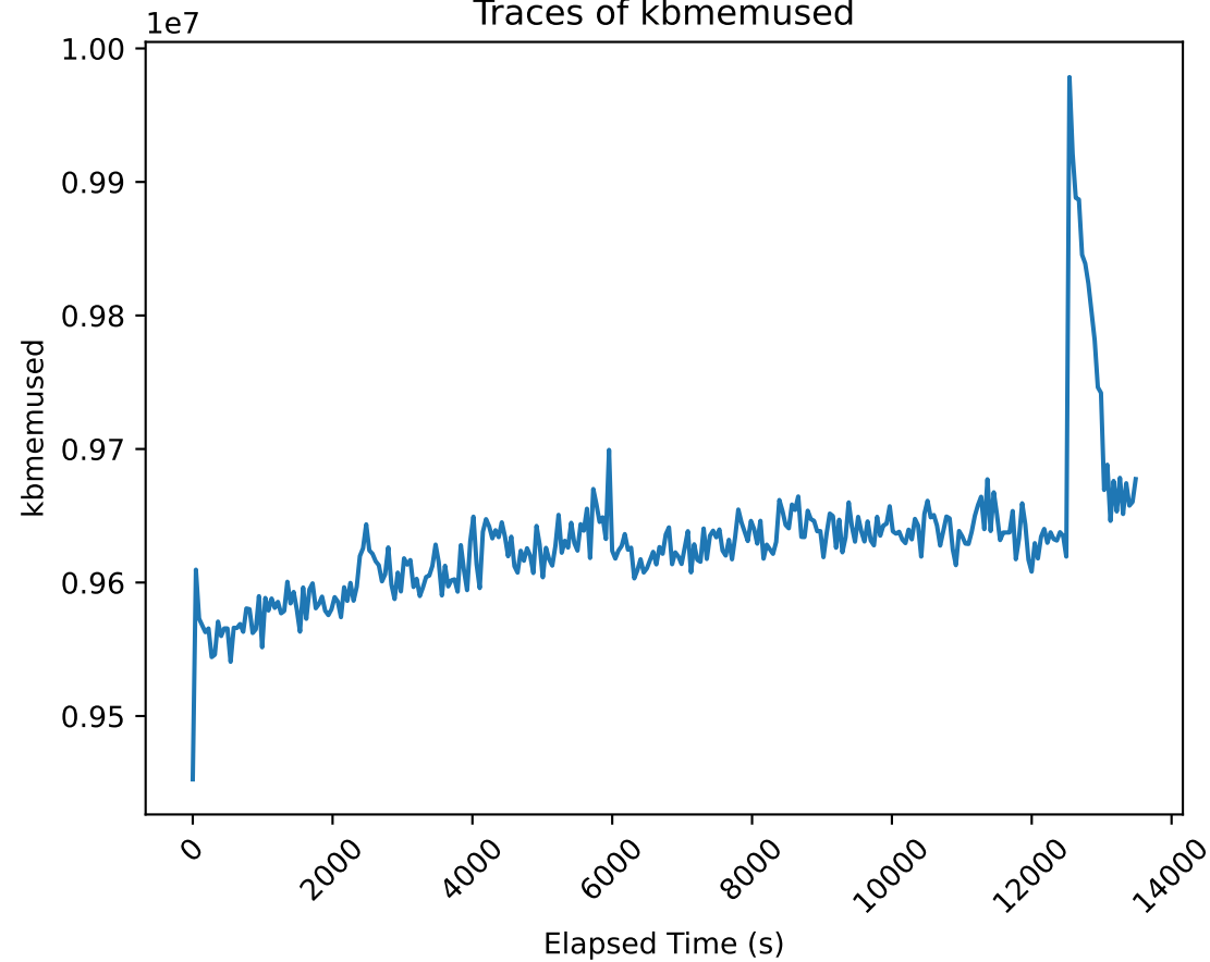
Traces of kbmemused
