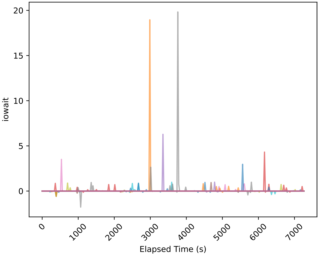
Traces of iowait for each cpu with utilization reaches 100%
